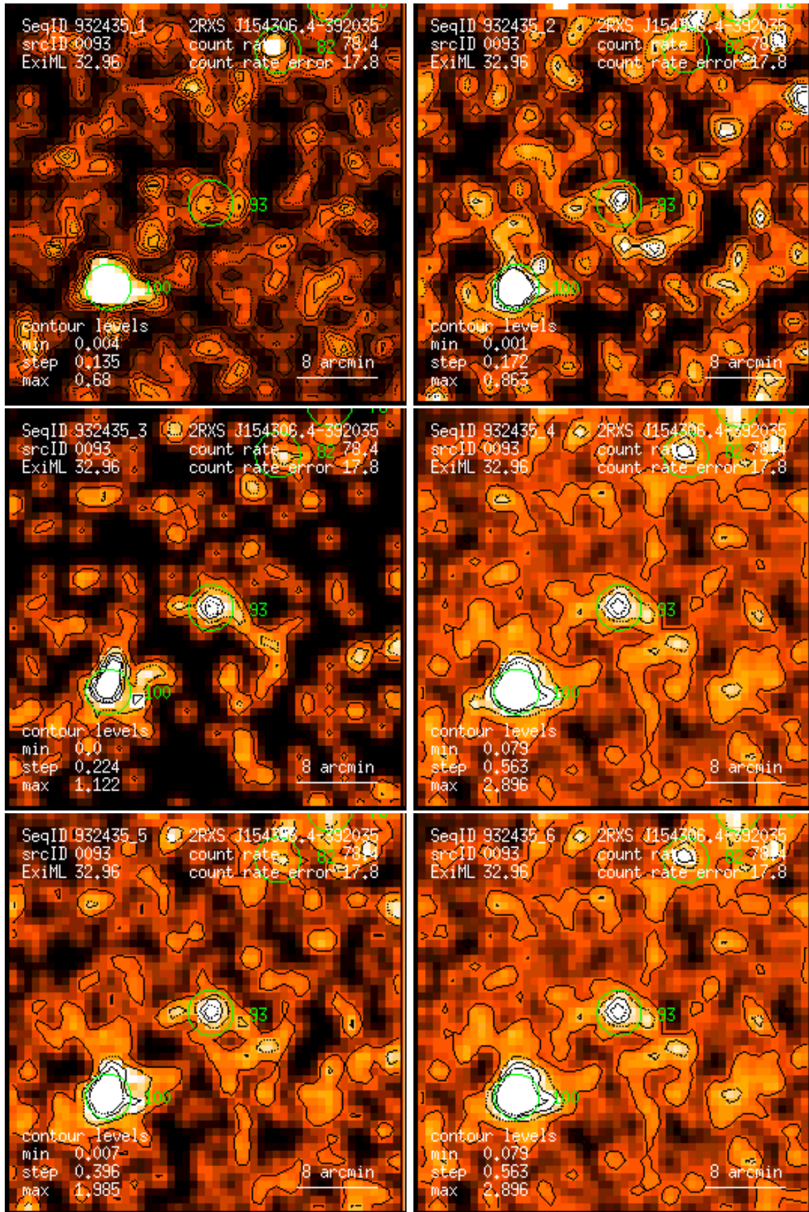
Figure 93: RASS 932435: detection 0093: band rate images, Gaussian filter: (1) PSPC channels 11 – 41, (2) 52 – 90, (3) 91 – 201, (4) 11 – 235, (5) 52 – 201, (6) 11 – 201. Broad band rates in counts/ks. Band rate contour levels in counts/ks/arcmin 2 .
