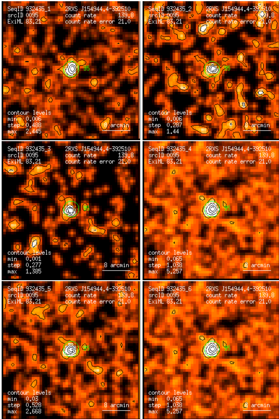
Figure 95: RASS 932435: detection 0095: band rate images, Gaussian filter: (1) PSPC channels 11 – 41, (2) 52 – 90, (3) 91 – 201, (4) 11 – 235, (5) 52 – 201, (6) 11 – 201. Broad band rates in counts/ks. Band rate contour levels in counts/ks/arcmin 2 .
