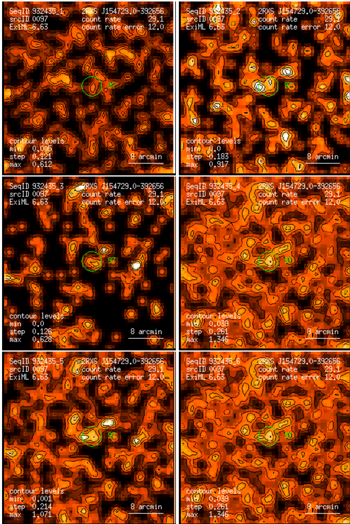
Figure 97: RASS 932435: detection 0097: band rate images, Gaussian filter: (1) PSPC channels 11 – 41, (2) 52 – 90, (3) 91 – 201, (4) 11 – 235, (5) 52 – 201, (6) 11 – 201. Broad band rates in counts/ks. Band rate contour levels in counts/ks/arcmin 2 .
