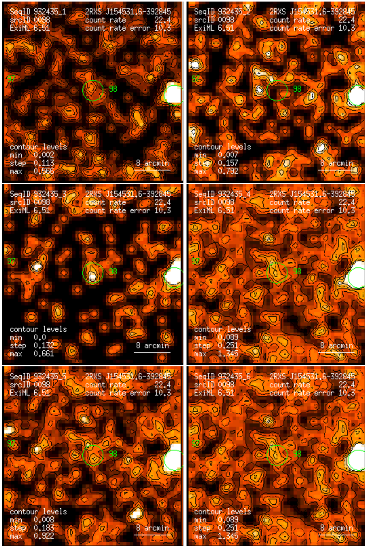
Figure 98: RASS 932435: detection 0098: band rate images, Gaussian filter: (1) PSPC channels 11 – 41, (2) 52 – 90, (3) 91 – 201, (4) 11 – 235, (5) 52 – 201, (6) 11 – 201. Broad band rates in counts/ks. Band rate contour levels in counts/ks/arcmin 2 .
