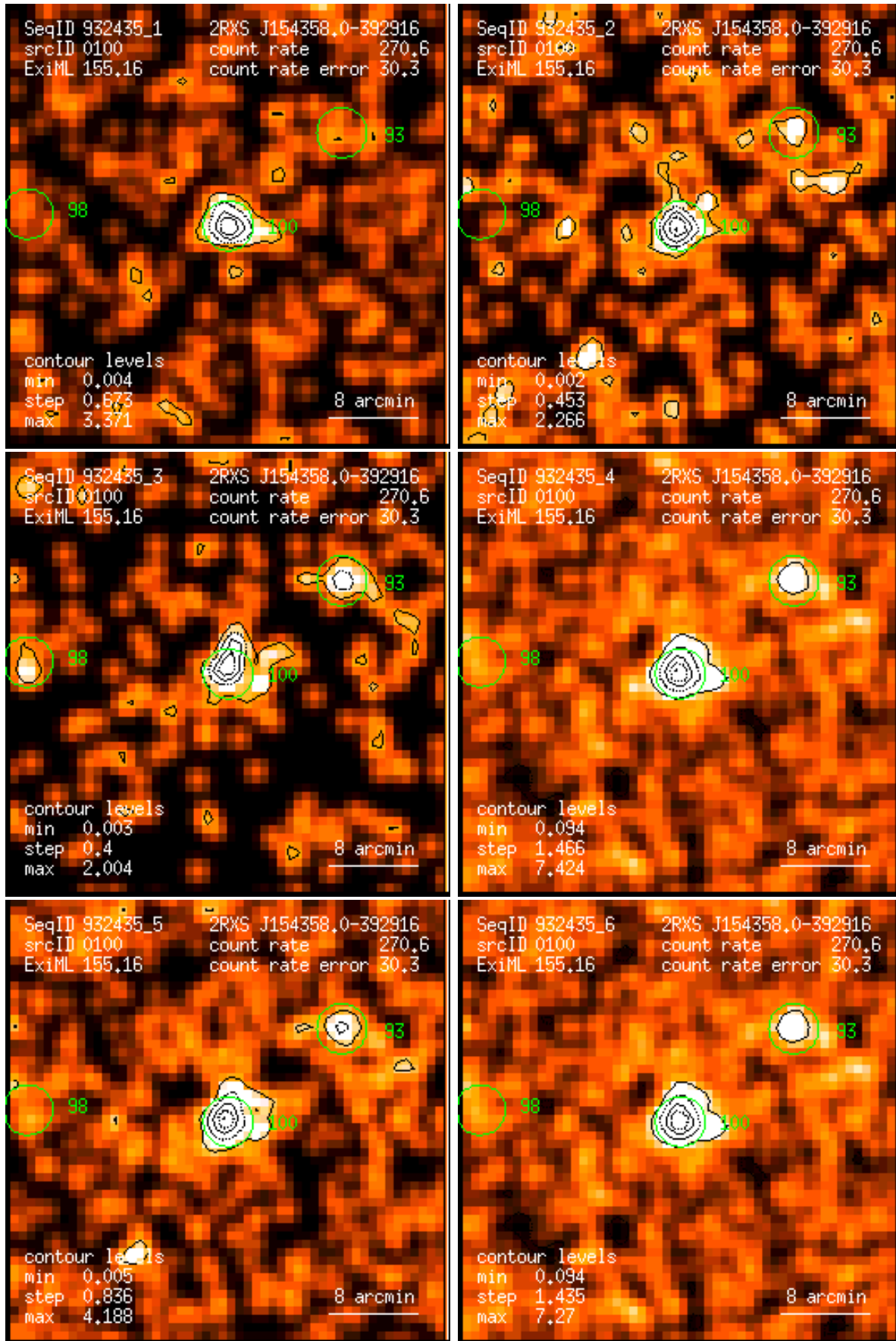
Figure 100: RASS 932435: detection 0100: band rate images, Gaussian filter: (1) PSPC channels 11 – 41, (2) 52 – 90, (3) 91 – 201, (4) 11 – 235, (5) 52 – 201, (6) 11 – 201. Broad band rates in counts/ks. Band rate contour levels in counts/ks/arcmin 2 .
