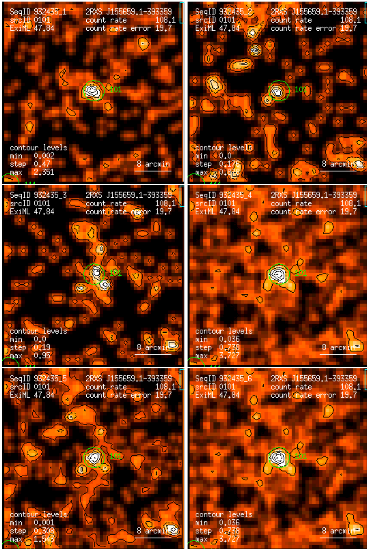
Figure 101: RASS 932435: detection 0101: band rate images, Gaussian filter: (1) PSPC channels 11 – 41, (2) 52 – 90, (3) 91 – 201, (4) 11 – 235, (5) 52 – 201, (6) 11 – 201. Broad band rates in counts/ks. Band rate contour levels in counts/ks/arcmin 2 .
