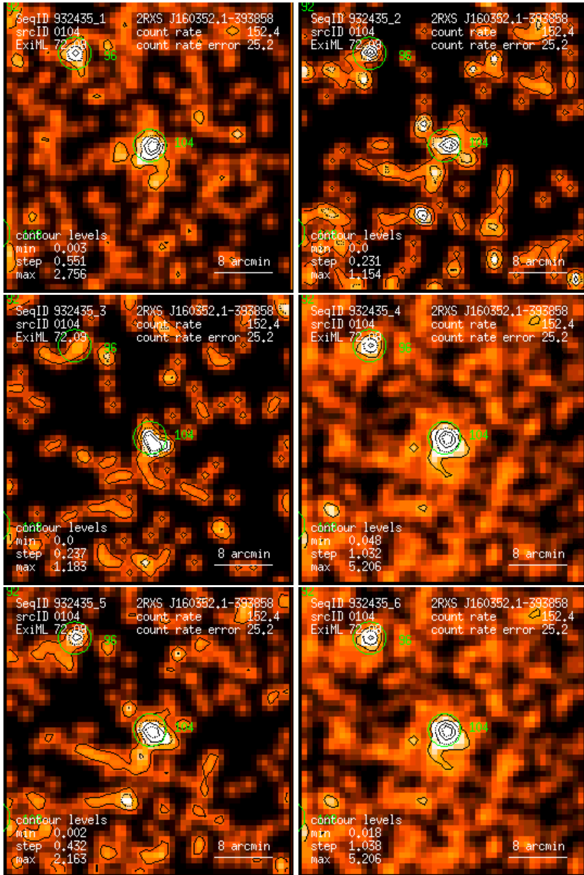
Figure 104: RASS 932435: detection 0104: band rate images, Gaussian filter: (1) PSPC channels 11 – 41, (2) 52 – 90, (3) 91 – 201, (4) 11 – 235, (5) 52 – 201, (6) 11 – 201. Broad band rates in counts/ks. Band rate contour levels in counts/ks/arcmin 2 .
