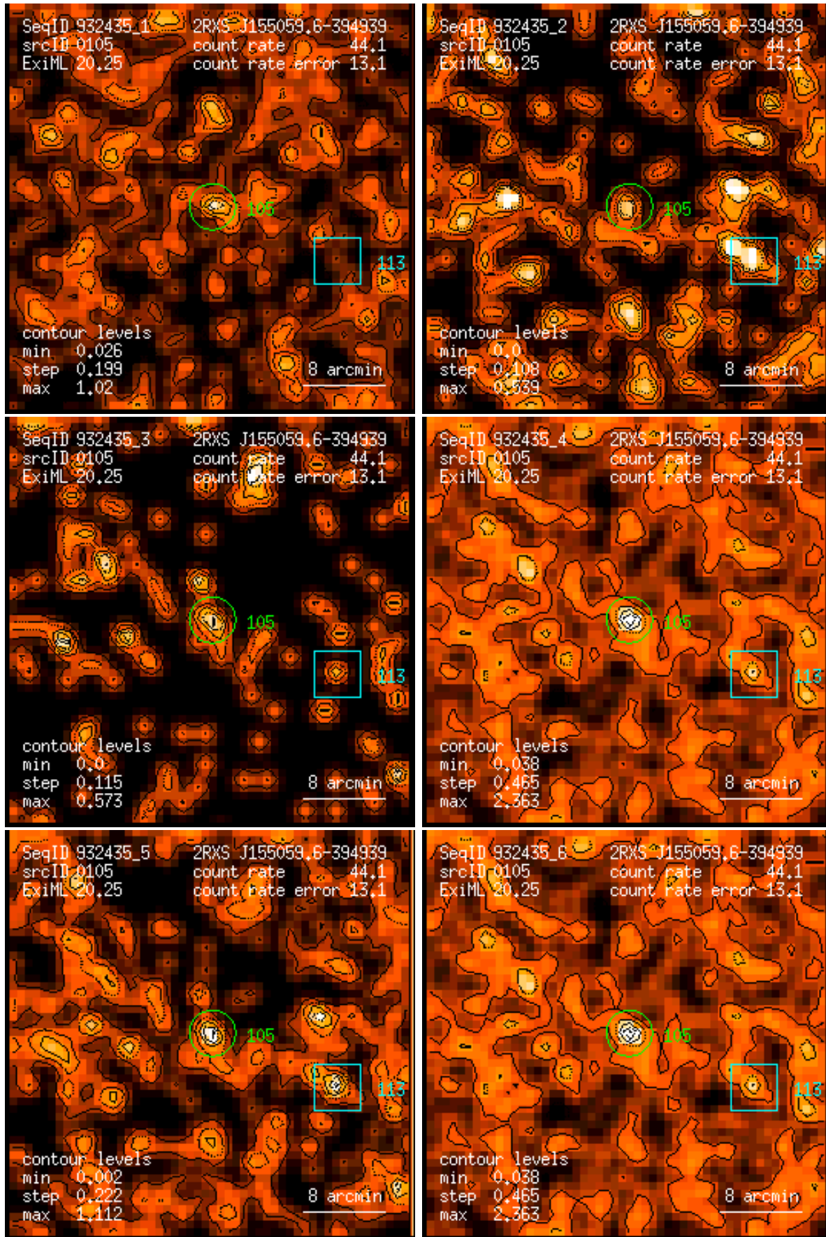
Figure 105: RASS 932435: detection 0105: band rate images, Gaussian filter: (1) PSPC channels 11 – 41, (2) 52 – 90, (3) 91 – 201, (4) 11 – 235, (5) 52 – 201, (6) 11 – 201. Broad band rates in counts/ks. Band rate contour levels in counts/ks/arcmin 2 .
