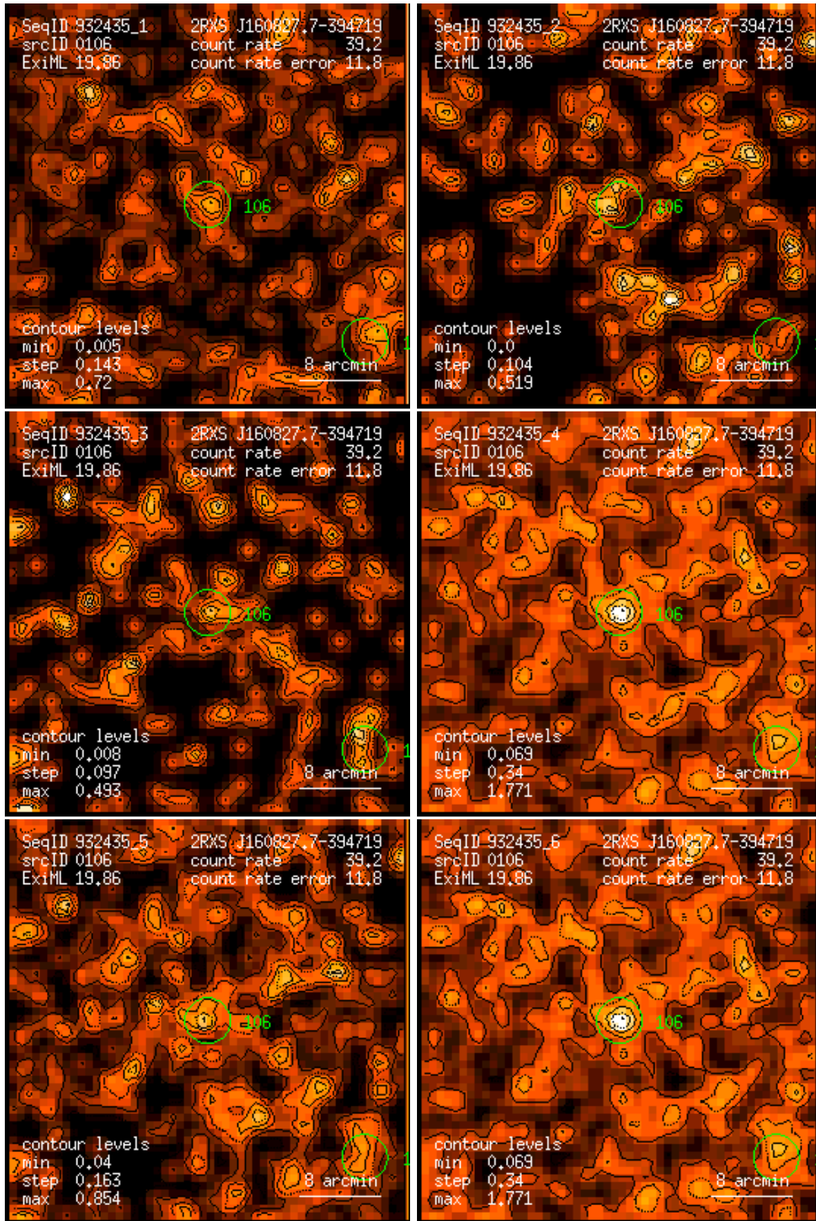
Figure 106: RASS 932435: detection 0106: band rate images, Gaussian filter: (1) PSPC channels 11 – 41, (2) 52 – 90, (3) 91 – 201, (4) 11 – 235, (5) 52 – 201, (6) 11 – 201. Broad band rates in counts/ks. Band rate contour levels in counts/ks/arcmin 2 .
