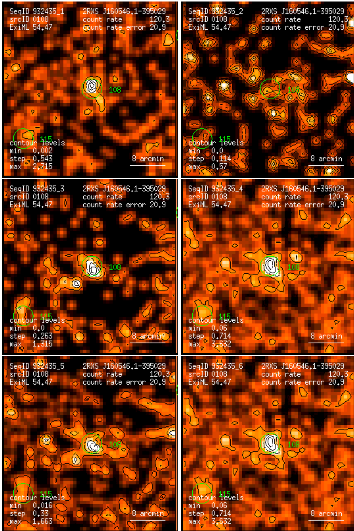
Figure 108: RASS 932435: detection 0108: band rate images, Gaussian filter: (1) PSPC channels 11 – 41, (2) 52 – 90, (3) 91 – 201, (4) 11 – 235, (5) 52 – 201, (6) 11 – 201. Broad band rates in counts/ks. Band rate contour levels in counts/ks/arcmin 2 .
