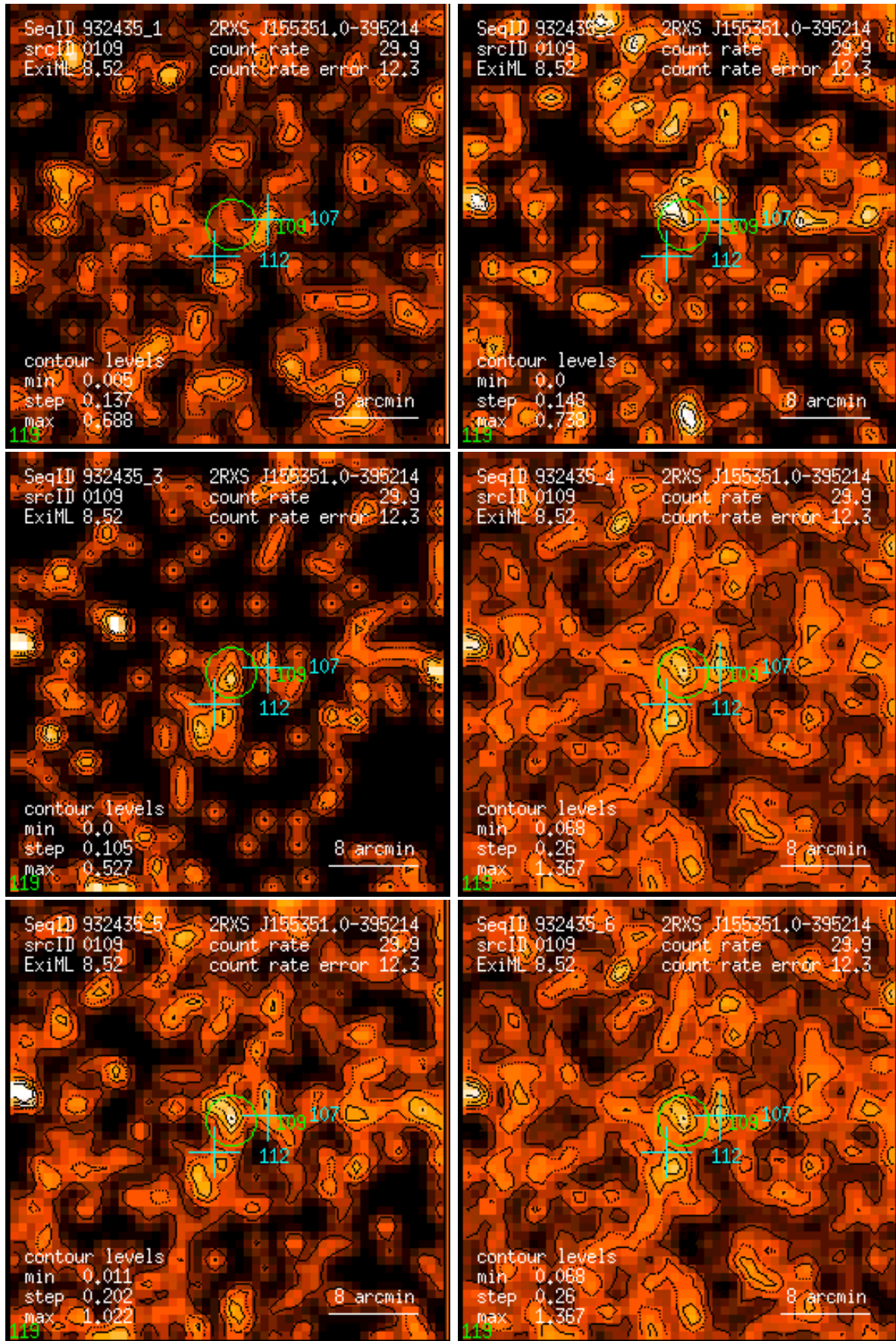
Figure 109: RASS 932435: detection 0109: band rate images, Gaussian filter: (1) PSPC channels 11 – 41, (2) 52 – 90, (3) 91 – 201, (4) 11 – 235, (5) 52 – 201, (6) 11 – 201. Broad band rates in counts/ks. Band rate contour levels in counts/ks/arcmin 2 .
