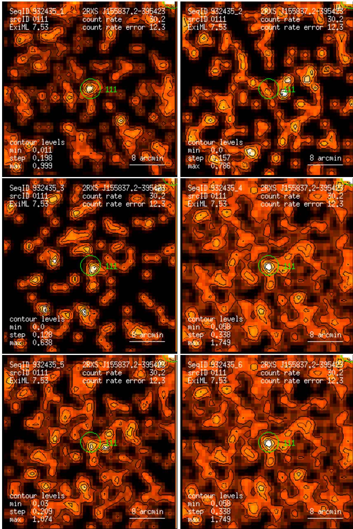
Figure 111: RASS 932435: detection 0111: band rate images, Gaussian filter: (1) PSPC channels 11 – 41, (2) 52 – 90, (3) 91 – 201, (4) 11 – 235, (5) 52 – 201, (6) 11 – 201. Broad band rates in counts/ks. Band rate contour levels in counts/ks/arcmin 2 .
