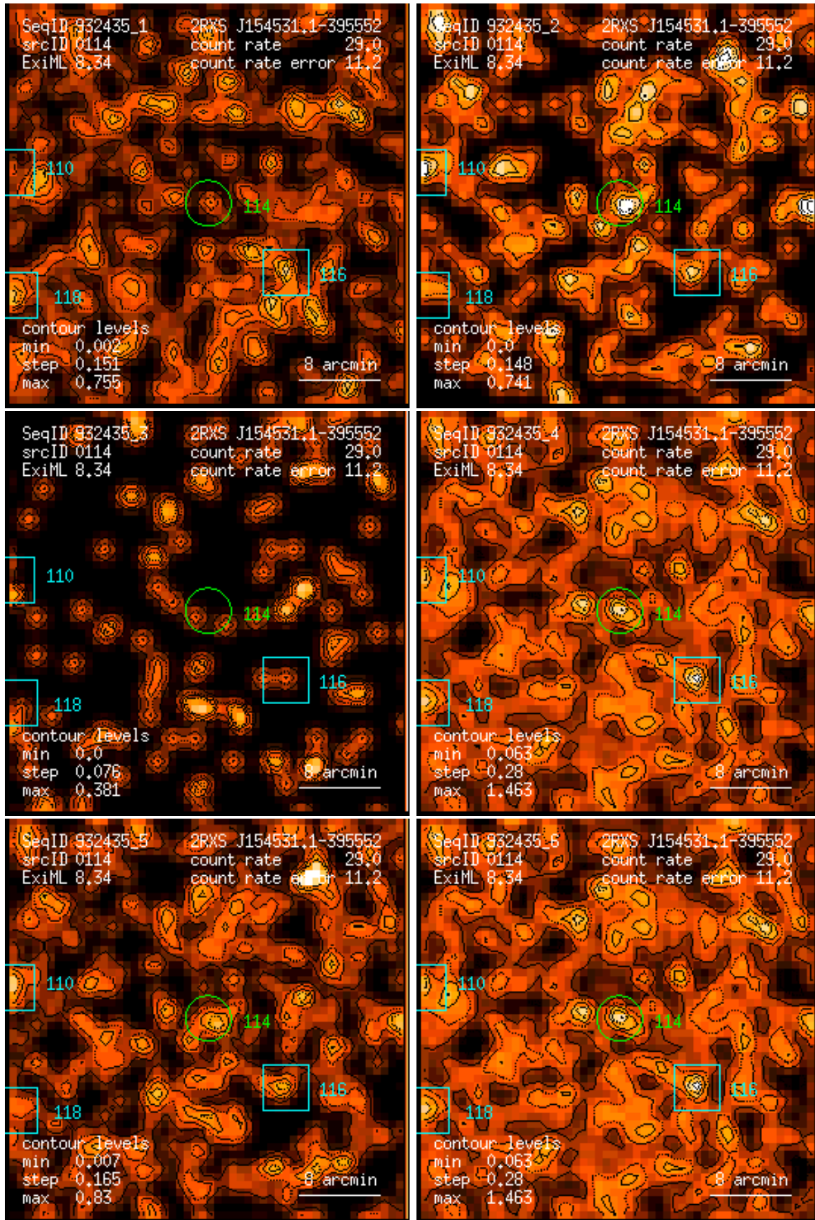
Figure 114: RASS 932435: detection 0114: band rate images, Gaussian filter: (1) PSPC channels 11 – 41, (2) 52 – 90, (3) 91 – 201, (4) 11 – 235, (5) 52 – 201, (6) 11 – 201. Broad band rates in counts/ks. Band rate contour levels in counts/ks/arcmin 2 .
