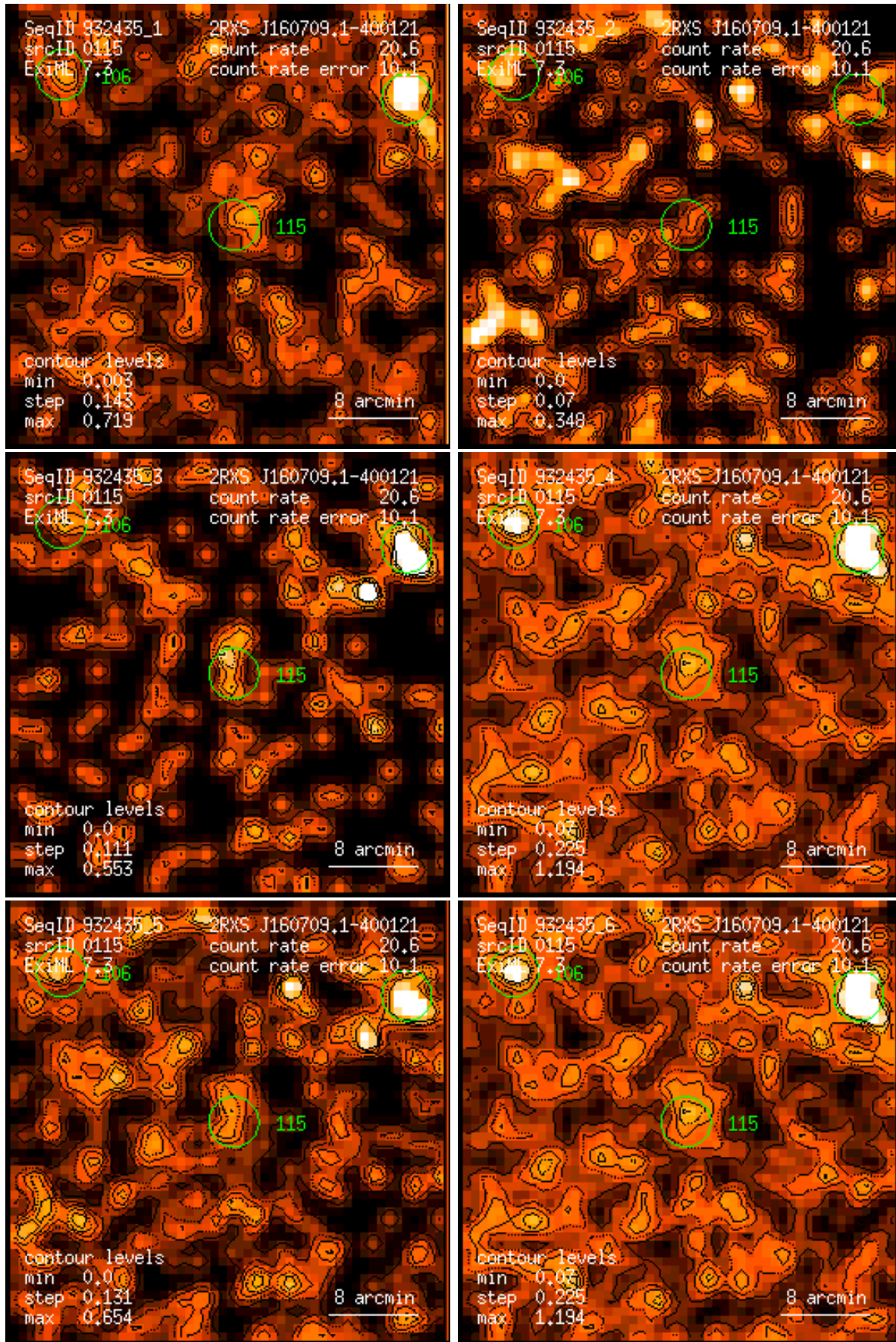
Figure 115: RASS 932435: detection 0115: band rate images, Gaussian filter: (1) PSPC channels 11 – 41, (2) 52 – 90, (3) 91 – 201, (4) 11 – 235, (5) 52 – 201, (6) 11 – 201. Broad band rates in counts/ks. Band rate contour levels in counts/ks/arcmin 2 .
