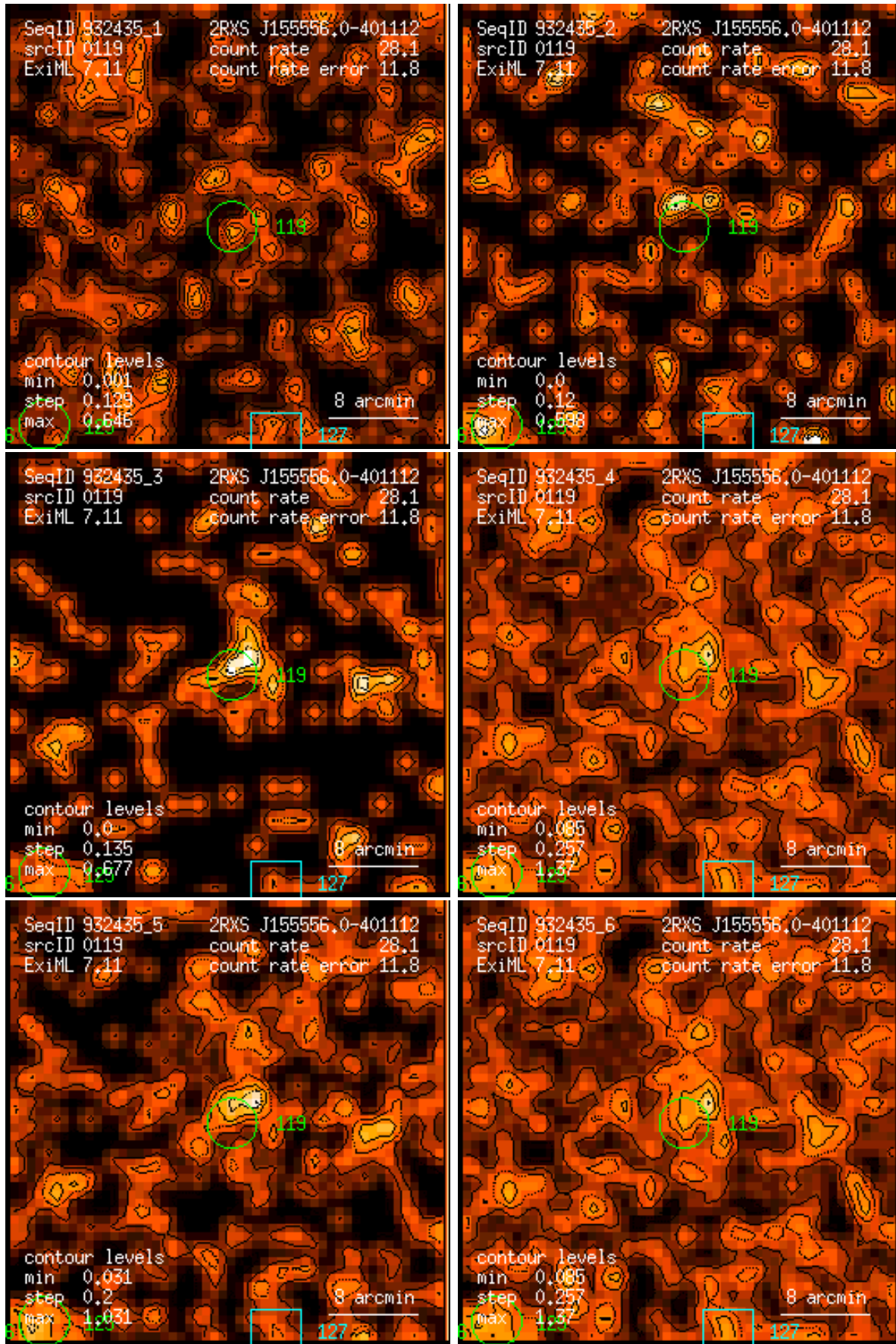
Figure 119: RASS 932435: detection 0119: band rate images, Gaussian filter: (1) PSPC channels 11 – 41, (2) 52 – 90, (3) 91 – 201, (4) 11 – 235, (5) 52 – 201, (6) 11 – 201. Broad band rates in counts/ks. Band rate contour levels in counts/ks/arcmin 2 .
