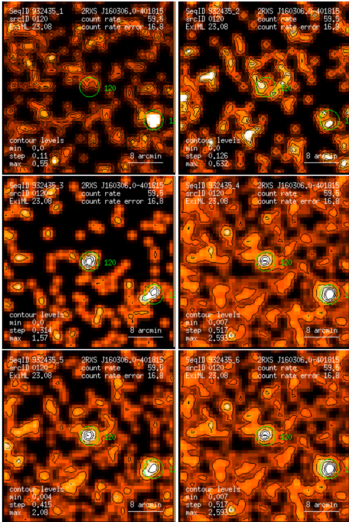
Figure 120: RASS 932435: detection 0120: band rate images, Gaussian filter: (1) PSPC channels 11 – 41, (2) 52 – 90, (3) 91 – 201, (4) 11 – 235, (5) 52 – 201, (6) 11 – 201. Broad band rates in counts/ks. Band rate contour levels in counts/ks/arcmin 2 .
