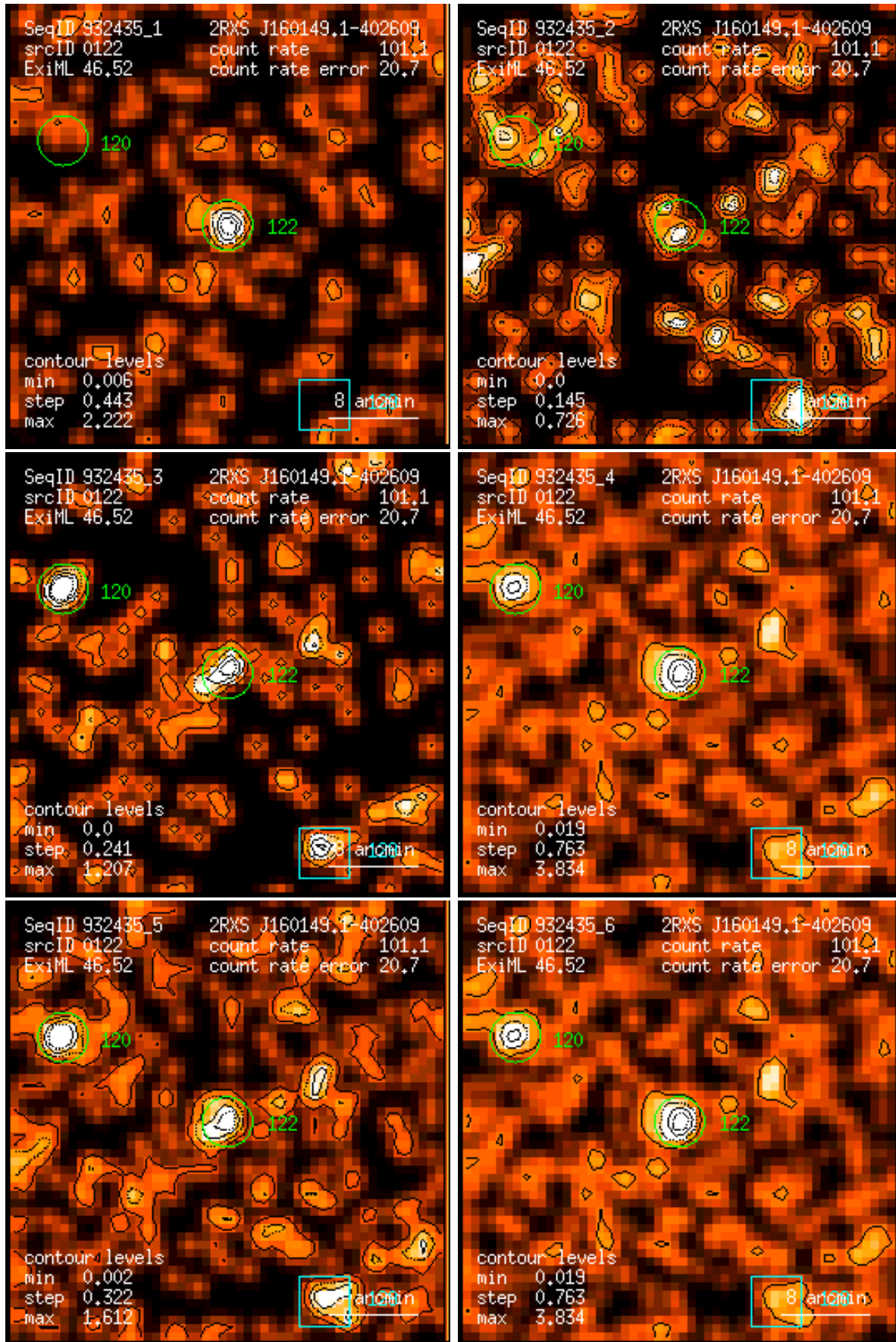
Figure 122: RASS 932435: detection 0122: band rate images, Gaussian filter: (1) PSPPC channels 11 – 41, (2) 52 – 90, (3) 91 – 201, (4) 11 – 235, (5) 52 – 201, (6) 11 – 201. Broad band rates in counts/ks. Band rate contour levels in counts/ks/arcmin 2 .
