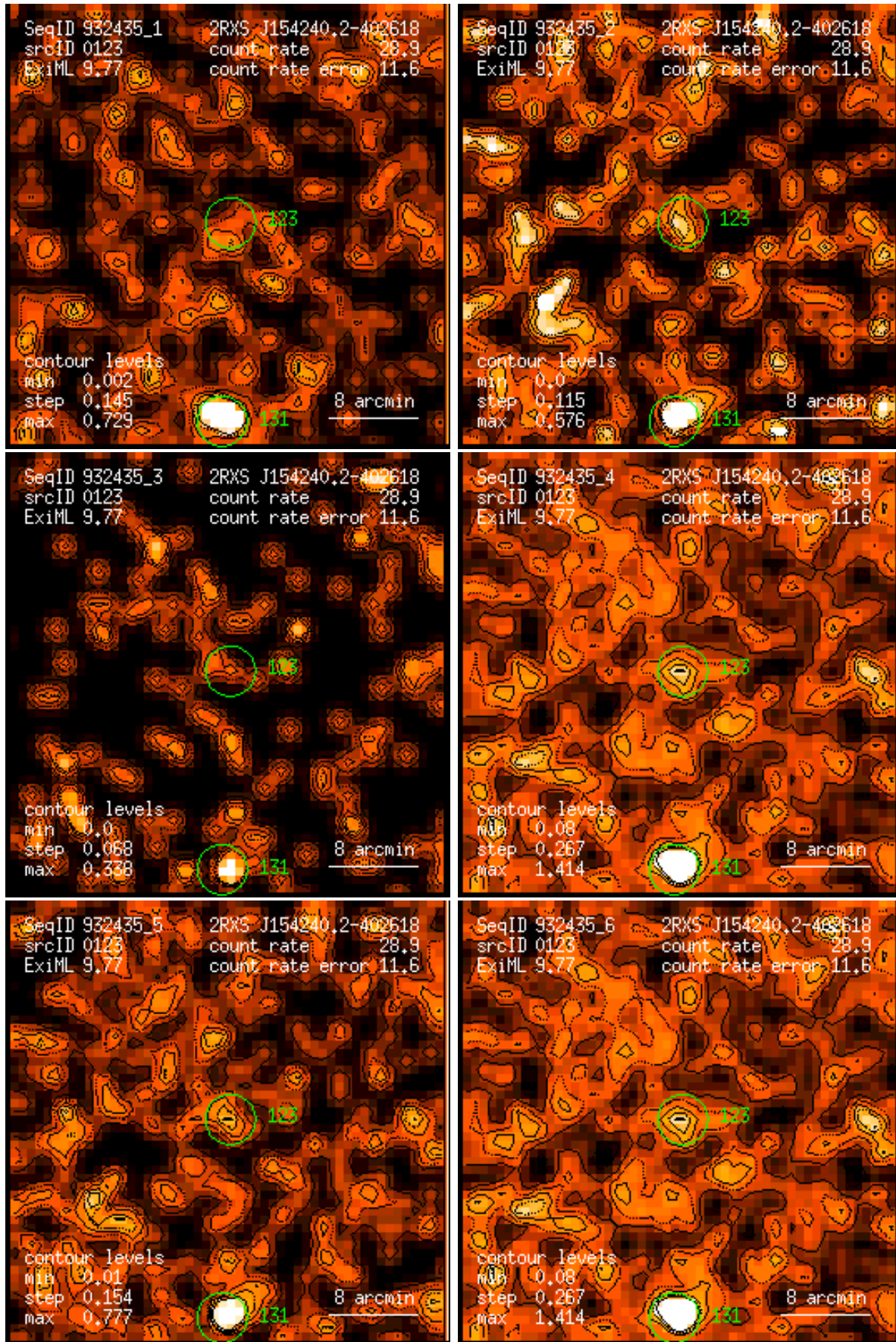
Figure 123: RASS 932435: detection 0123: band rate images, Gaussian filter: (1) PSPPC channels 11 – 41, (2) 52 – 90, (3) 91 – 201, (4) 11 – 235, (5) 52 – 201, (6) 11 – 201. Broad band rates in counts/ks. Band rate contour levels in counts/ks/arcmin 2 .
