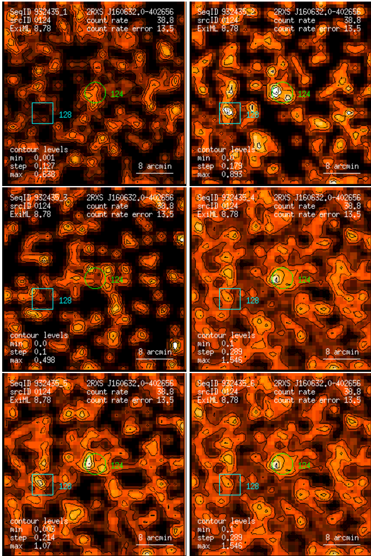
Figure 124: RASS 932435: detection 0124: band rate images, Gaussian filter: (1) PSPC channels 11 – 41, (2) 52 – 90, (3) 91 – 201, (4) 11 – 235, (5) 52 – 201, (6) 11 – 201. Broad band rates in counts/ks. Band rate contour levels in counts/ks/arcmin 2 .
