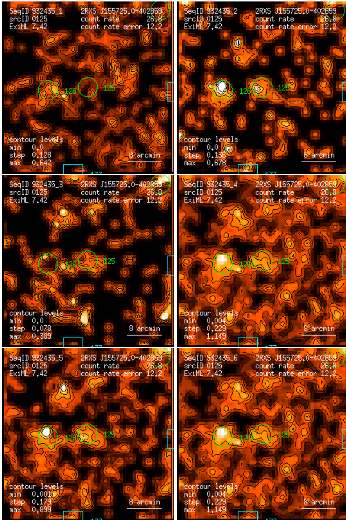
Figure 125: RASS 932435: detection 0125: band rate images, Gaussian filter: (1) PSPC channels 11 – 41, (2) 52 – 90, (3) 91 – 201, (4) 11 – 235, (5) 52 – 201, (6) 11 – 201. Broad band rates in counts/ks. Band rate contour levels in counts/ks/arcmin 2 .
