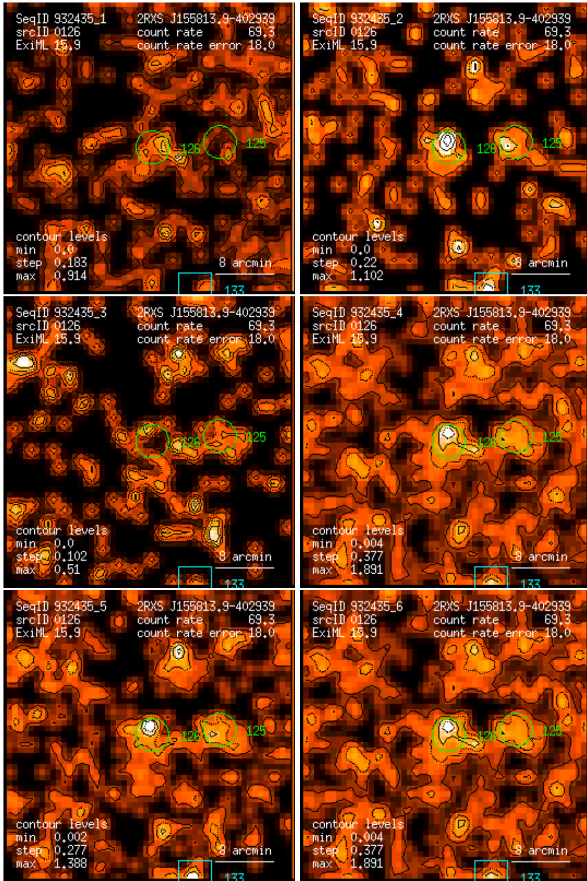
Figure 126: RASS 932435: detection 0126: band rate images, Gaussian filter: (1) PSPC channels 11 – 41, (2) 52 – 90, (3) 91 – 201, (4) 11 – 235, (5) 52 – 201, (6) 11 – 201. Broad band rates in counts/ks. Band rate contour levels in counts/ks/arcmin 2 .
