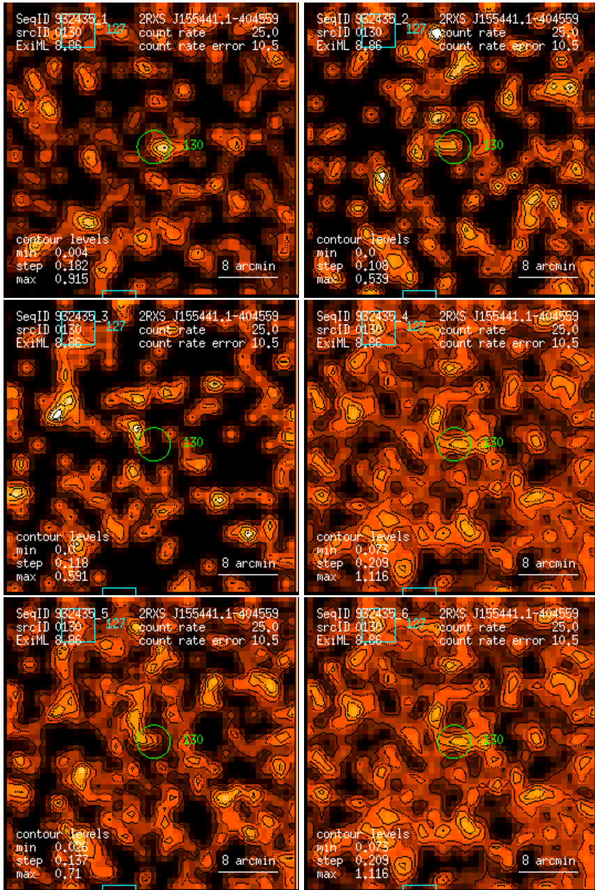
Figure 130: RASS 932435: detection 0130: band rate images, Gaussian filter: (1) PSPC channels 11 – 41, (2) 52 – 90, (3) 91 – 201, (4) 11 – 235, (5) 52 – 201, (6) 11 – 201. Broad band rates in counts/ks. Band rate contour levels in counts/ks/arcmin 2 .
