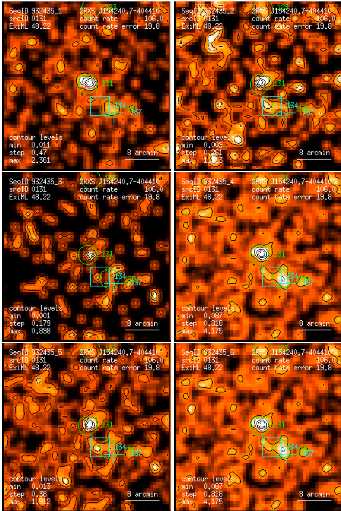
Figure 131: RASS 932435: detection 0131: band rate images, Gaussian filter: (1) PSPC channels 11 – 41, (2) 52 – 90, (3) 91 – 201, (4) 11 – 235, (5) 52 – 201, (6) 11 – 201. Broad band rates in counts/ks. Band rate contour levels in counts/ks/arcmin 2 .
