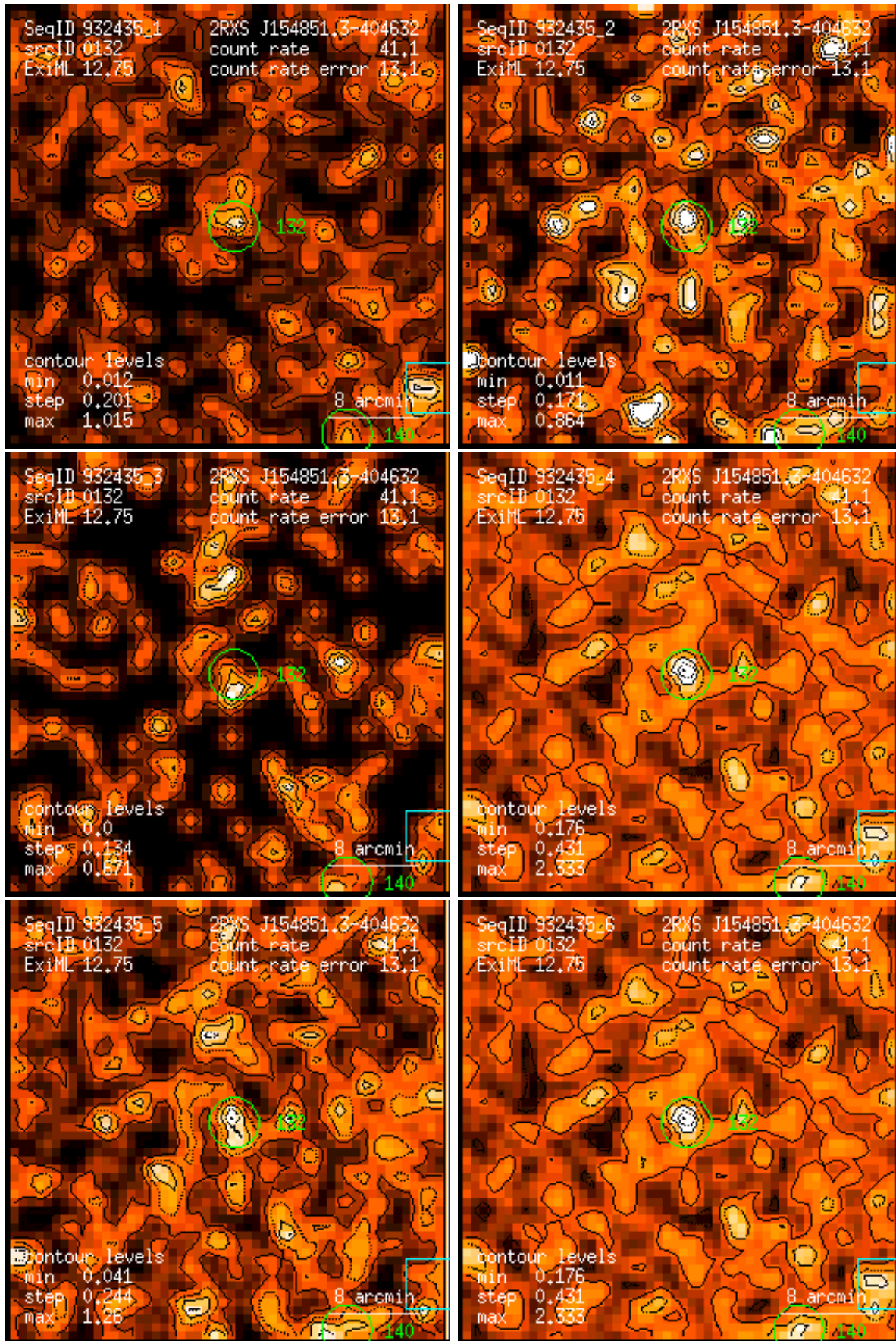
Figure 132: RASS 932435: detection 0132: band rate images, Gaussian filter: (1) PSPC channels 11 – 41, (2) 52 – 90, (3) 91 – 201, (4) 11 – 235, (5) 52 – 201, (6) 11 – 201. Broad band rates in counts/ks. Band rate contour levels in counts/ks/arcmin 2 .
