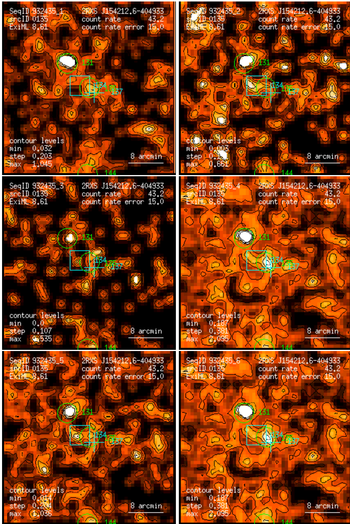
Figure 135: RASS 932435: detection 0135: band rate images, Gaussian filter: (1) PSPC channels 11 – 41, (2) 52 – 90, (3) 91 – 201, (4) 11 – 235, (5) 52 – 201, (6) 11 – 201. Broad band rates in counts/ks. Band rate contour levels in counts/ks/arcmin 2 .
