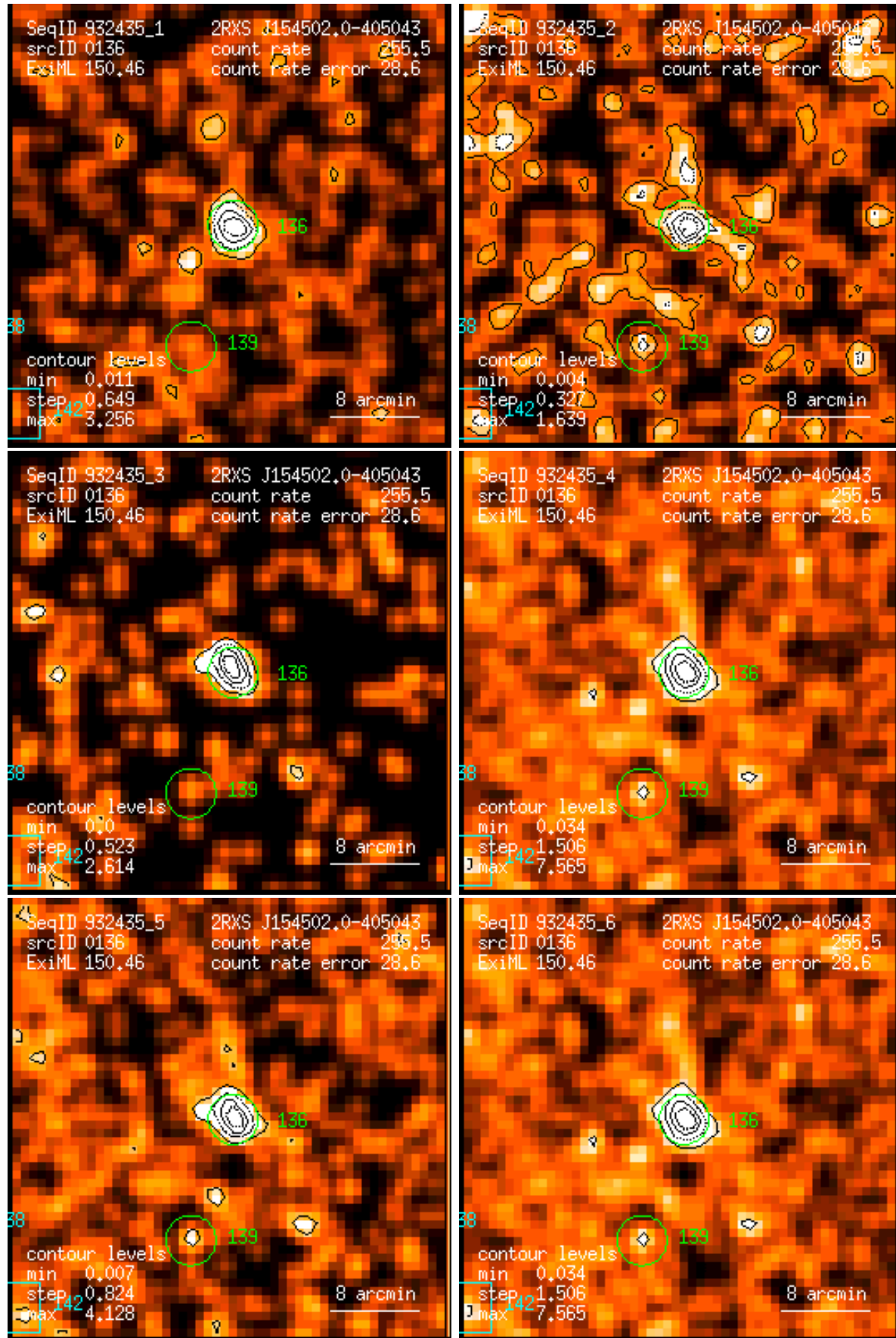
Figure 136: RASS 932435: detection 0136: band rate images, Gaussian filter: (1) PSPC channels 11 – 41, (2) 52 – 90, (3) 91 – 201, (4) 11 – 235, (5) 52 – 201, (6) 11 – 201. Broad band rates in counts/ks. Band rate contour levels in counts/ks/arcmin 2 .
