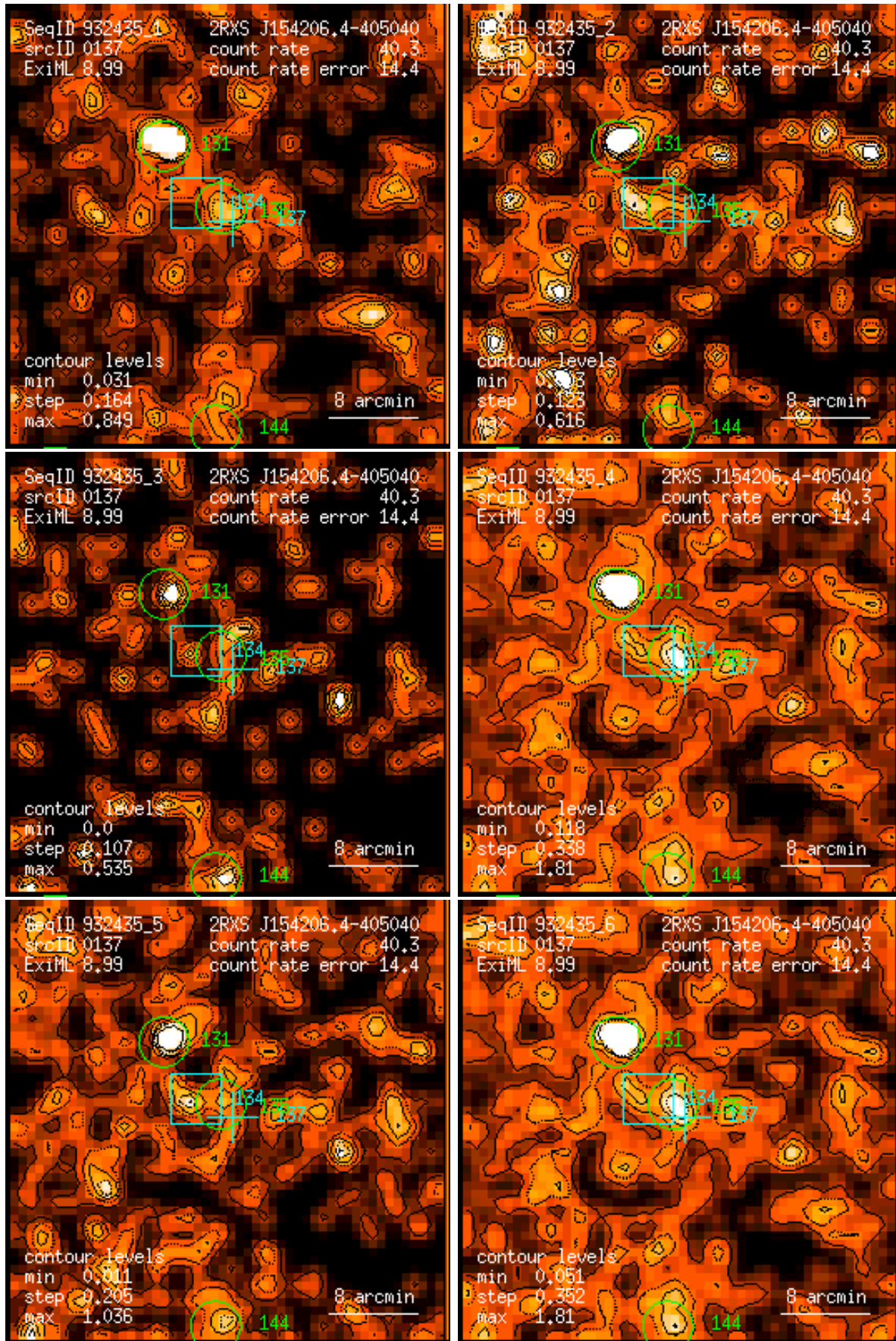
Figure 137: RASS 932435: detection 0137: band rate images, Gaussian filter: (1) PSPC channels 11 – 41, (2) 52 – 90, (3) 91 – 201, (4) 11 – 235, (5) 52 – 201, (6) 11 – 201. Broad band rates in counts/ks. Band rate contour levels in counts/ks/arcmin 2 .
