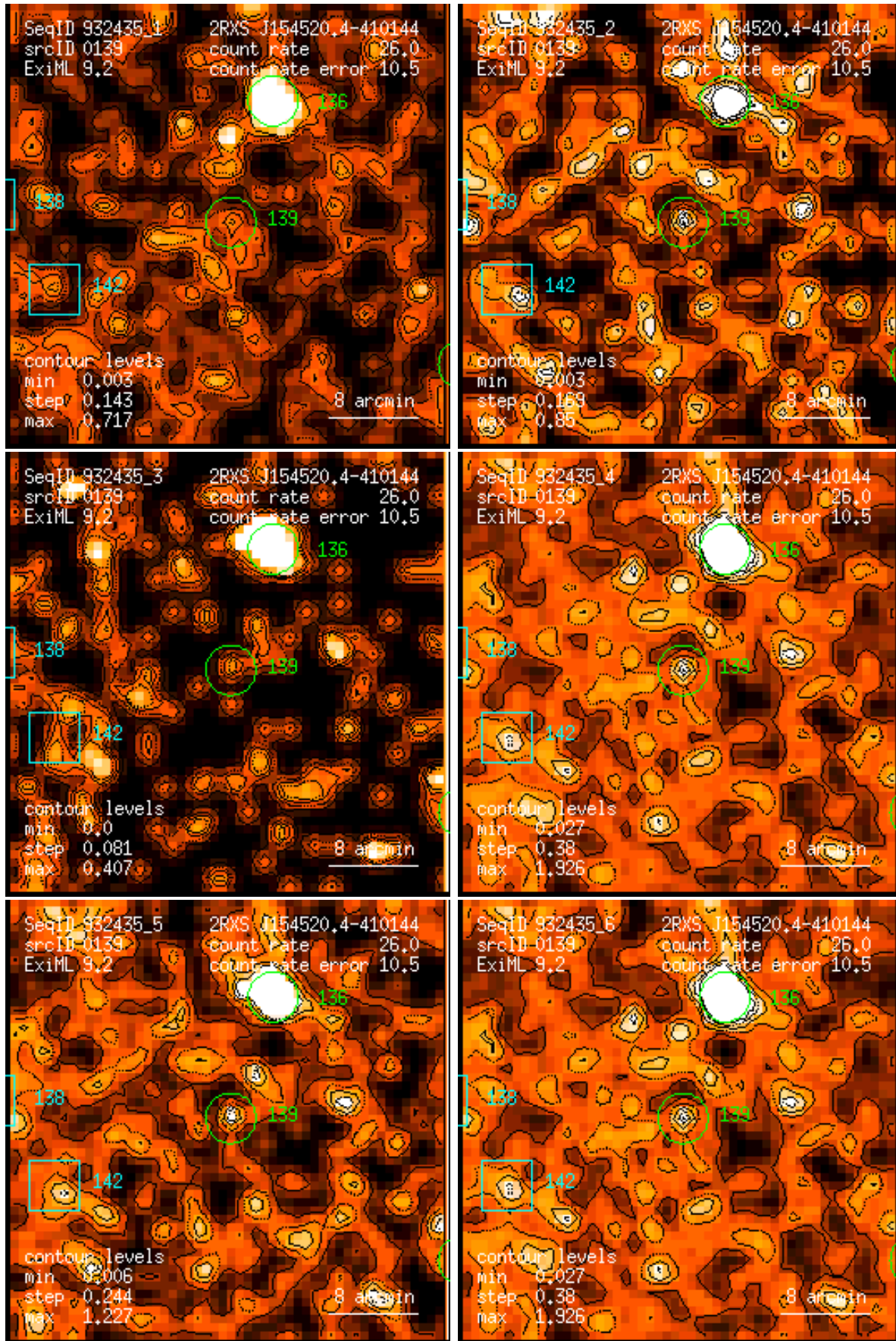
Figure 139: RASS 932435: detection 0139: band rate images, Gaussian filter: (1) PSPC channels 11 – 41, (2) 52 – 90, (3) 91 – 201, (4) 11 – 235, (5) 52 – 201, (6) 11 – 201. Broad band rates in counts/ks. Band rate contour levels in counts/ks/arcmin 2 .
