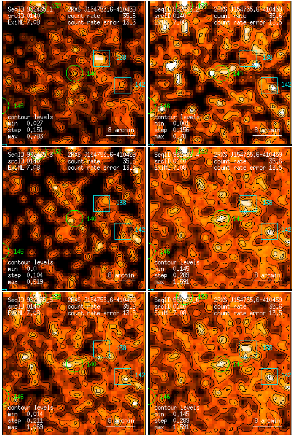
Figure 140: RASS 932435: detection 0140: band rate images, Gaussian filter: (1) PSPC channels 11 – 41, (2) 52 – 90, (3) 91 – 201, (4) 11 – 235, (5) 52 – 201, (6) 11 – 201. Broad band rates in counts/ks. Band rate contour levels in counts/ks/arcmin 2 .
