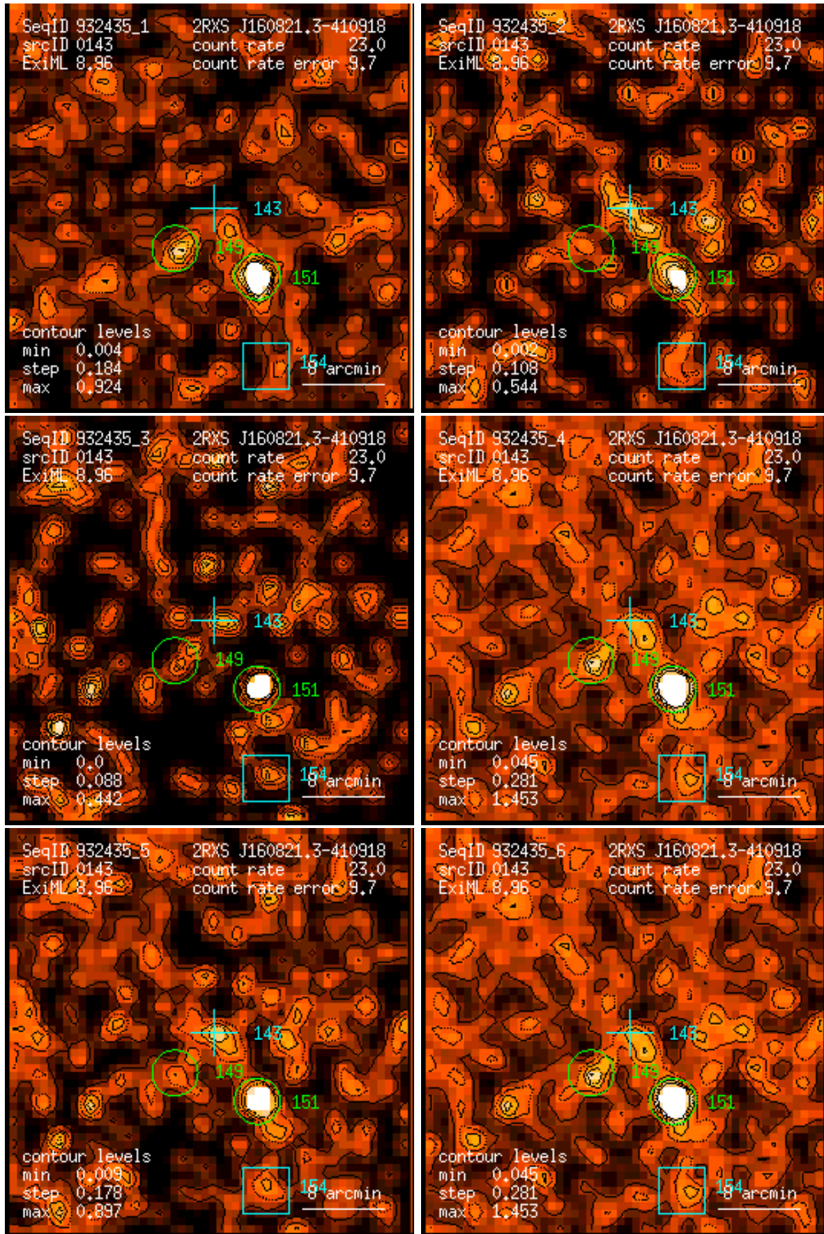
Figure 143: RASS 932435: detection 0143: band rate images, Gaussian filter: (1) PSPC channels 11 – 41, (2) 52 – 90, (3) 91 – 201, (4) 11 – 235, (5) 52 – 201, (6) 11 – 201. Broad band rates in counts/ks. Band rate contour levels in counts/ks/arcmin 2 .
