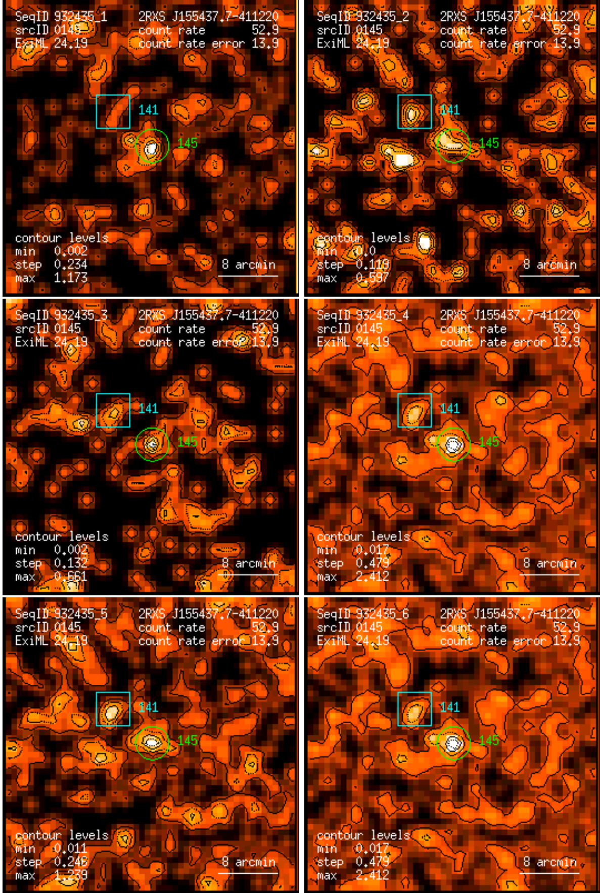
Figure 145: RASS 932435: detection 0145: band rate images, Gaussian filter: (1) PSPC channels 11 – 41, (2) 52 – 90, (3) 91 – 201, (4) 11 – 235, (5) 52 – 201, (6) 11 – 201. Broad band rates in counts/ks. Band rate contour levels in counts/ks/arcmin 2 .
