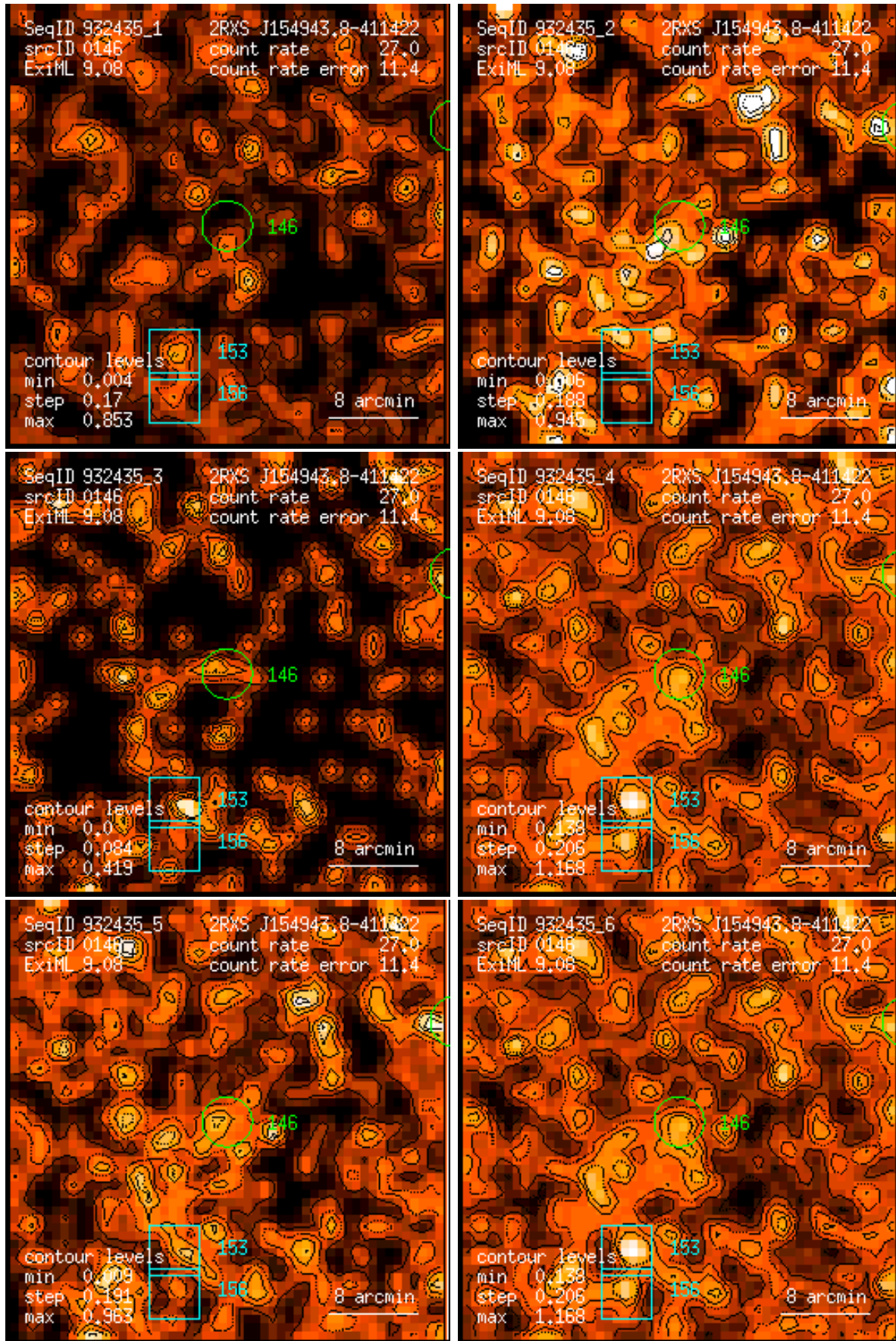
Figure 146: RASS 932435: detection 0146: band rate images, Gaussian filter: (1) PSPC channels 11 – 41, (2) 52 – 90, (3) 91 – 201, (4) 11 – 235, (5) 52 – 201, (6) 11 – 201. Broad band rates in counts/ks. Band rate contour levels in counts/ks/arcmin 2 .
