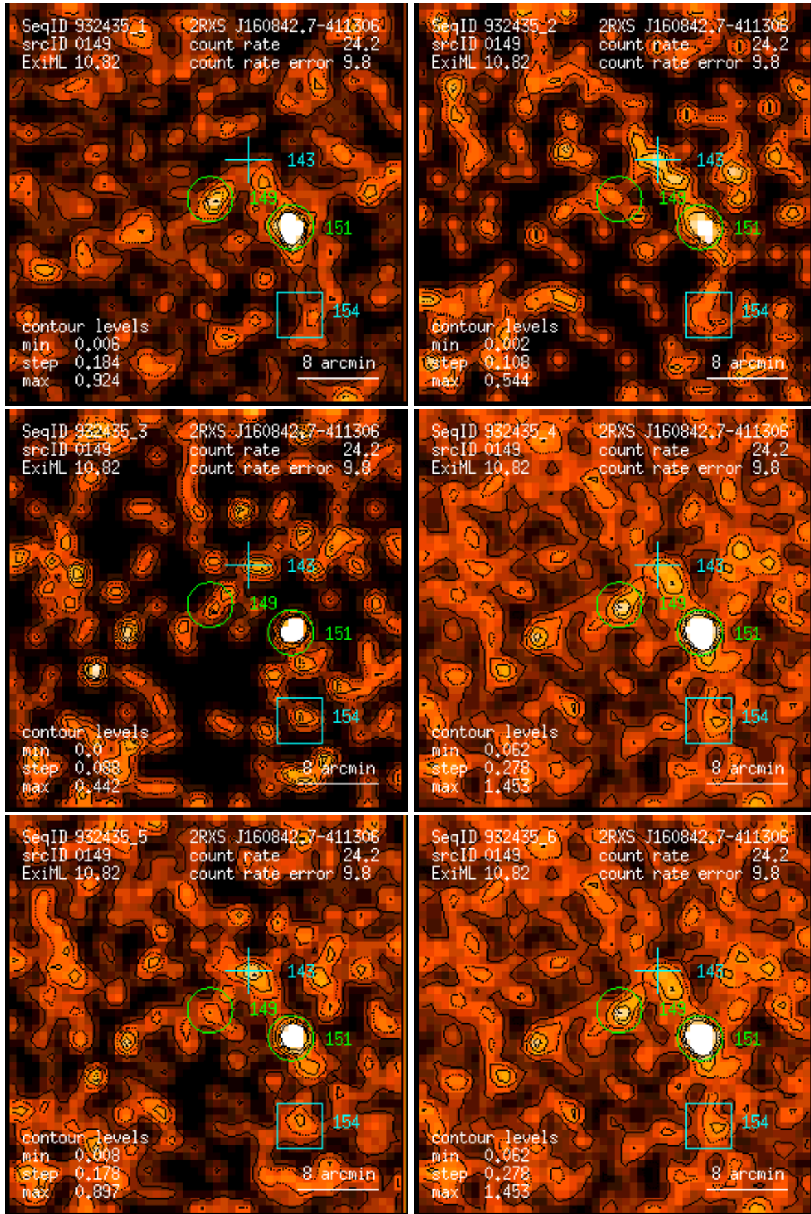
Figure 149: RASS 932435: detection 0149: band rate images, Gaussian filter: (1) PSPC channels 11 – 41, (2) 52 – 90, (3) 91 – 201, (4) 11 – 235, (5) 52 – 201, (6) 11 – 201. Broad band rates in counts/ks. Band rate contour levels in counts/ks/arcmin 2 .
