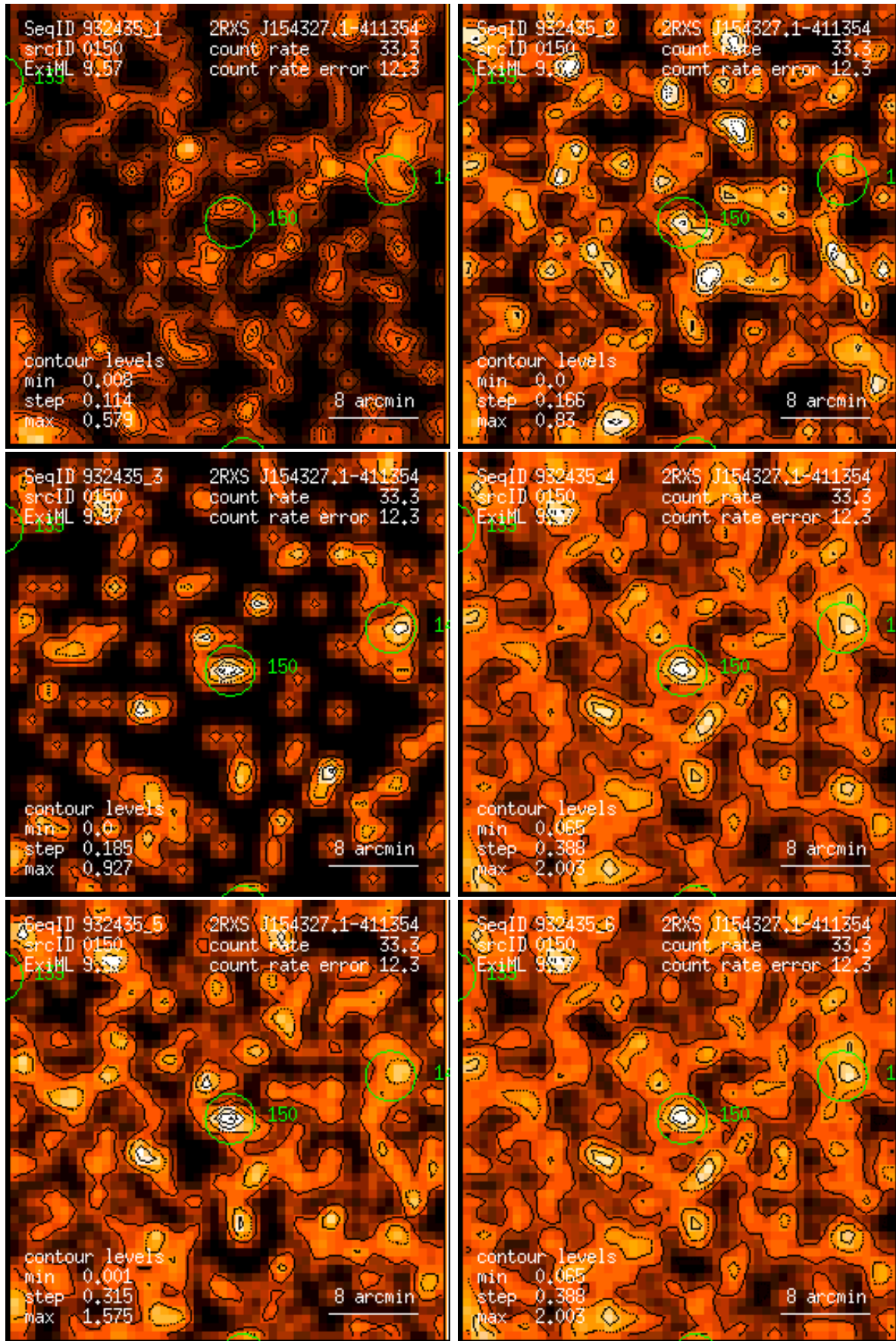
Figure 150: RASS 932435: detection 0150: band rate images, Gaussian filter: (1) PSPC channels 11 – 41, (2) 52 – 90, (3) 91 – 201, (4) 11 – 235, (5) 52 – 201, (6) 11 – 201. Broad band rates in counts/ks. Band rate contour levels in counts/ks/arcmin 2 .
