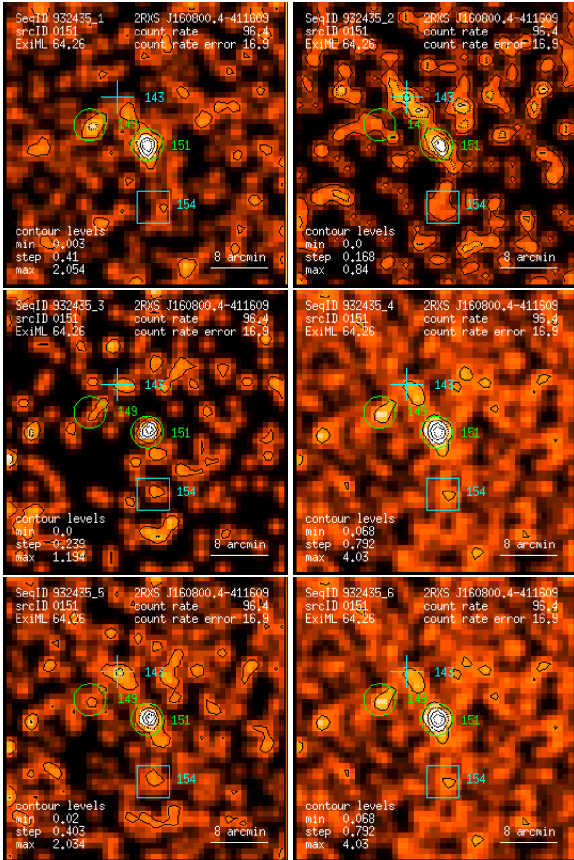
Figure 151: RASS 932435: detection 0151: band rate images, Gaussian filter: (1) PSPC channels 11 – 41, (2) 52 – 90, (3) 91 – 201, (4) 11 – 235, (5) 52 – 201, (6) 11 – 201. Broad band rates in counts/ks. Band rate contour levels in counts/ks/arcmin 2 .
