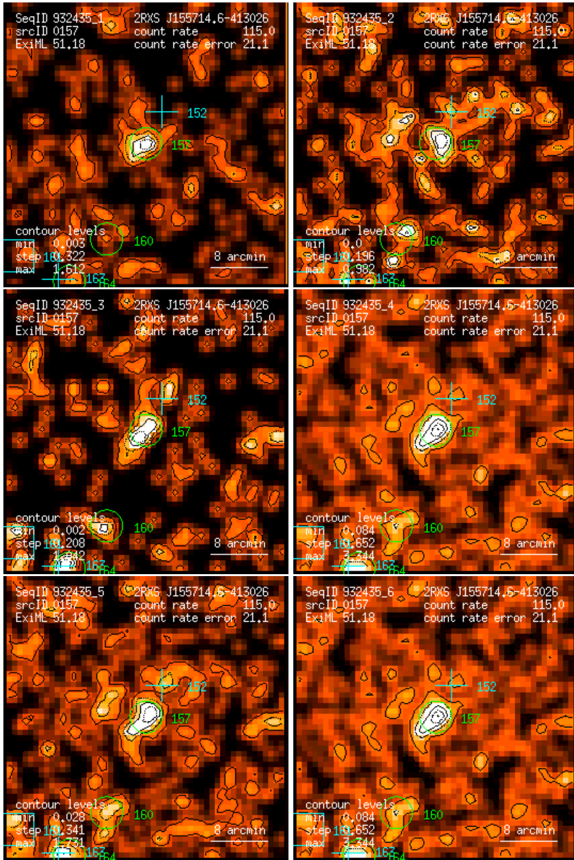
Figure 157: RASS 932435: detection 0157: band rate images, Gaussian filter: (1) PSPC channels 11 – 41, (2) 52 – 90, (3) 91 – 201, (4) 11 – 235, (5) 52 – 201, (6) 11 – 201. Broad band rates in counts/ks. Band rate contour levels in counts/ks/arcmin 2 .
