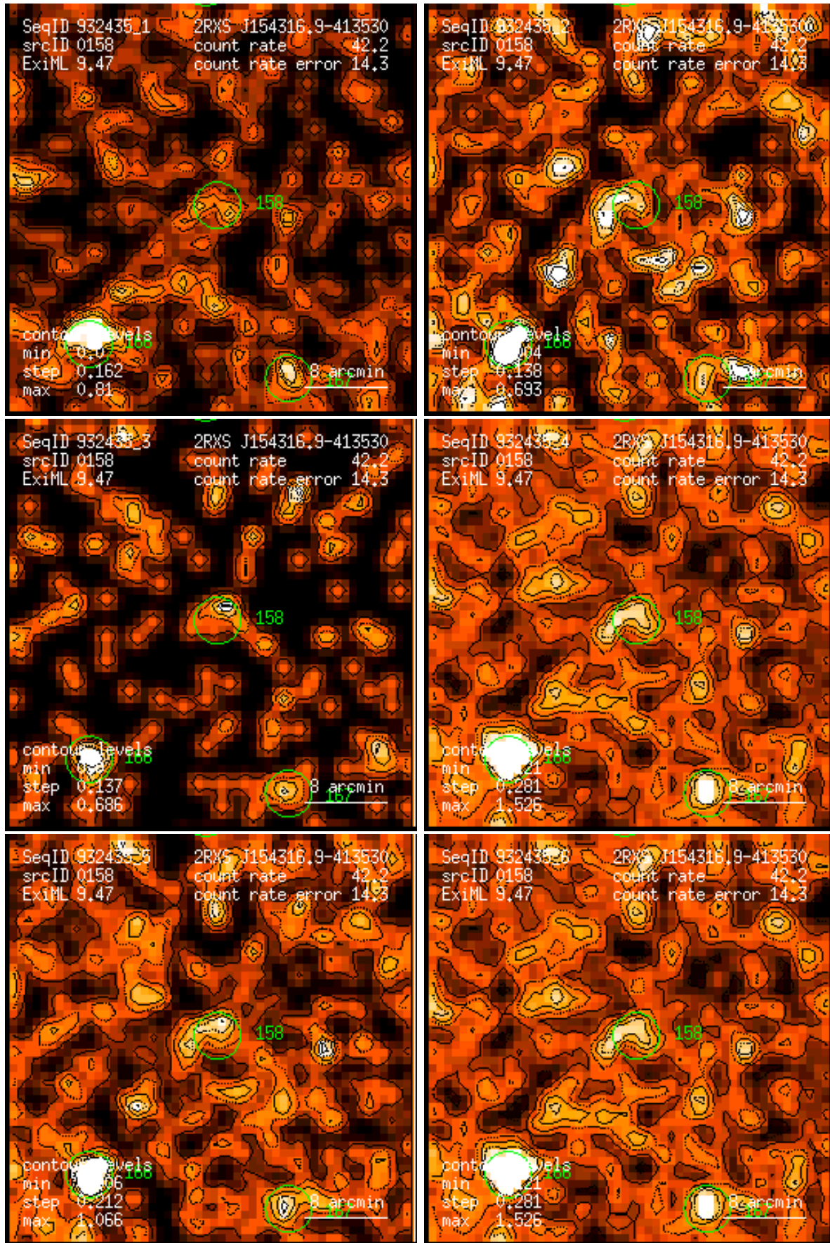
Figure 158: RASS 932435: detection 0158: band rate images, Gaussian filter: (1) PSPC channels 11 – 41, (2) 52 – 90, (3) 91 – 201, (4) 11 – 235, (5) 52 – 201, (6) 11 – 201. Broad band rates in counts/ks. Band rate contour levels in counts/ks/arcmin 2 .
