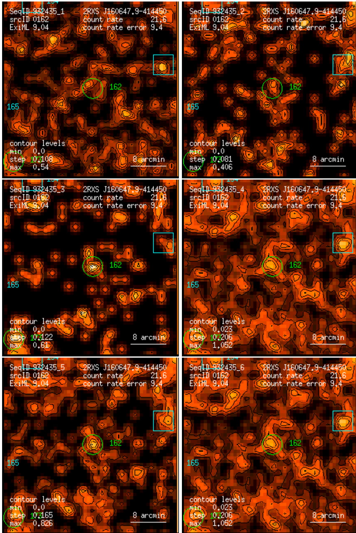
Figure 162: RASS 932435: detection 0162: band rate images, Gaussian filter: (1) PSPC channels 11 – 41, (2) 52 – 90, (3) 91 – 201, (4) 11 – 235, (5) 52 – 201, (6) 11 – 201. Broad band rates in counts/ks. Band rate contour levels in counts/ks/arcmin 2 .
