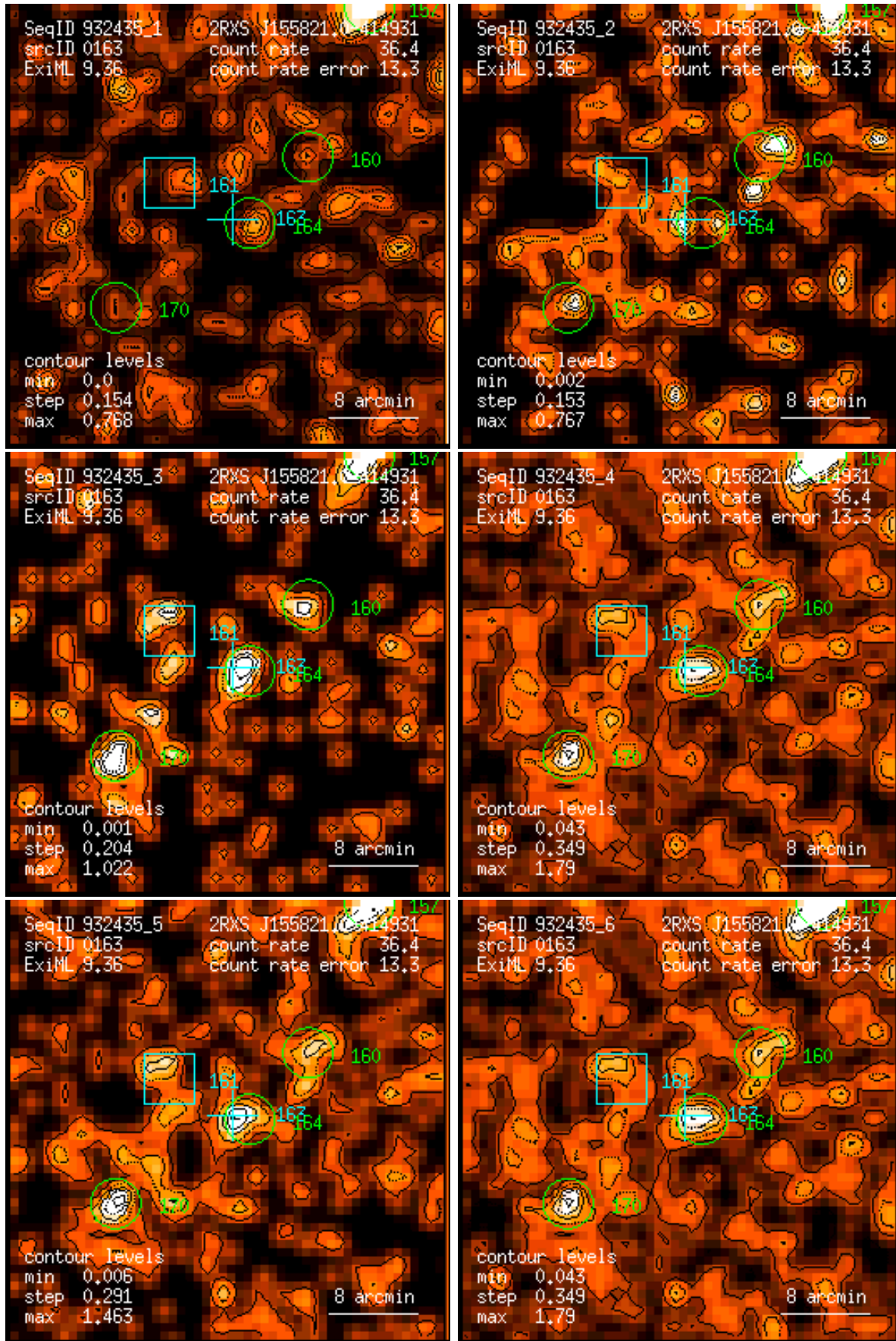
Figure 163: RASS 932435: detection 0163: band rate images, Gaussian filter: (1) PSPC channels 11 – 41, (2) 52 – 90, (3) 91 – 201, (4) 11 – 235, (5) 52 – 201, (6) 11 – 201. Broad band rates in counts/ks. Band rate contour levels in counts/ks/arcmin 2 .
