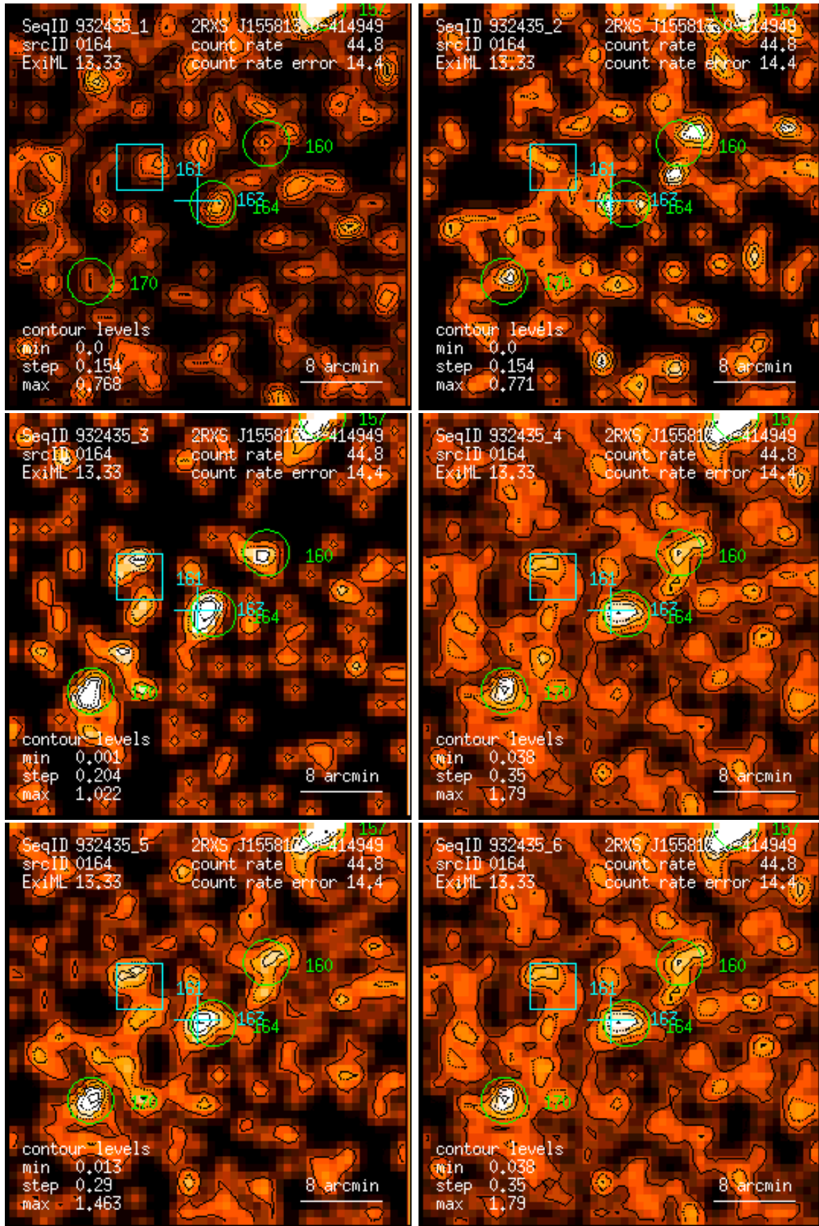
Figure 164: RASS 932435: detection 0164: band rate images, Gaussian filter: (1) PSPC channels 11 – 41, (2) 52 – 90, (3) 91 – 201, (4) 11 – 235, (5) 52 – 201, (6) 11 – 201. Broad band rates in counts/ks. Band rate contour levels in counts/ks/arcmin 2 .
