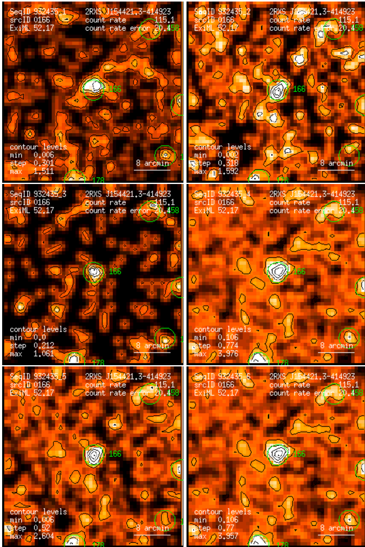
Figure 166: RASS 932435: detection 0166: band rate images, Gaussian filter: (1) PSPC channels 11 – 41, (2) 52 – 90, (3) 91 – 201, (4) 11 – 235, (5) 52 – 201, (6) 11 – 201. Broad band rates in counts/ks. Band rate contour levels in counts/ks/arcmin 2 .
