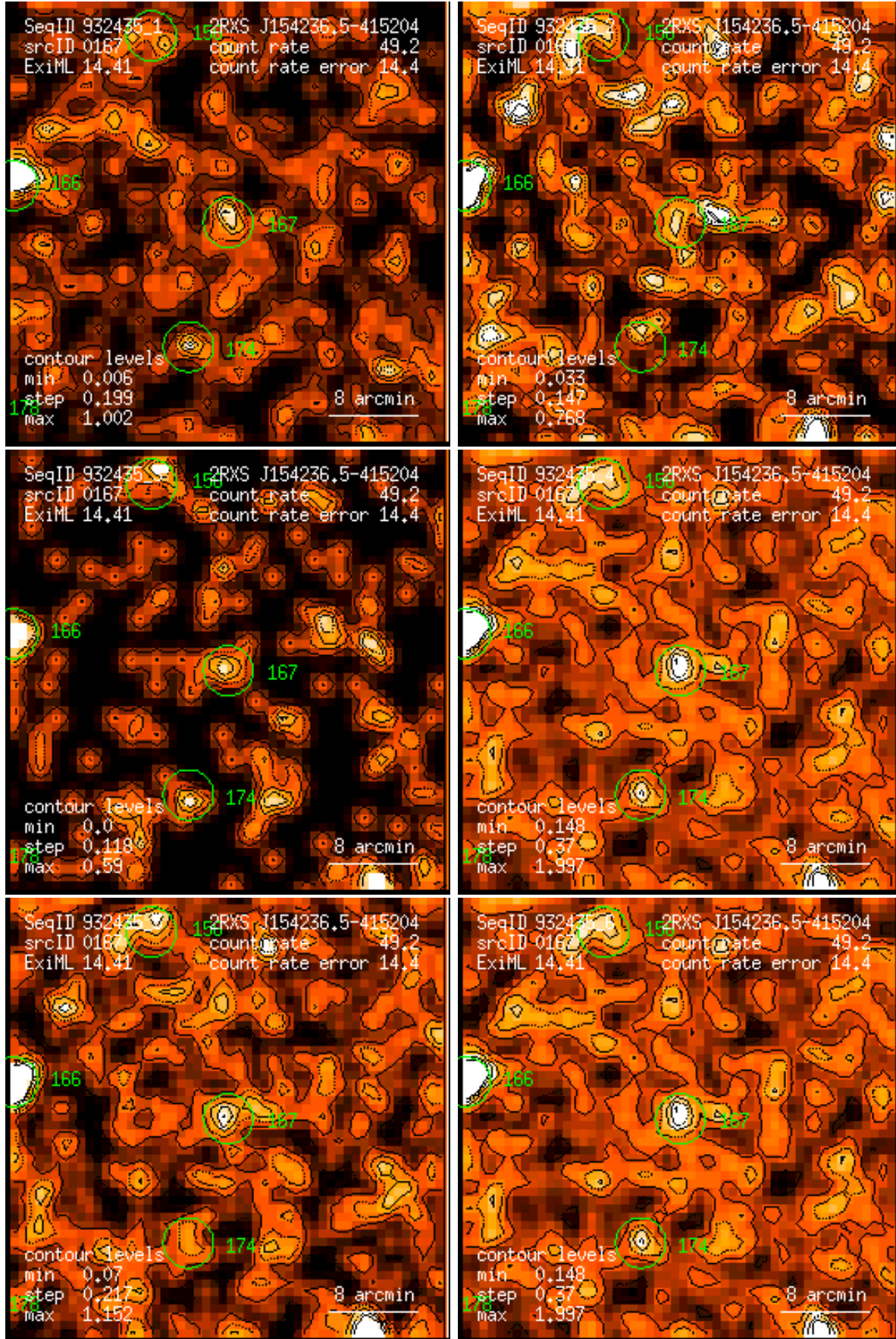
Figure 167: RASS 932435: detection 0167: band rate images, Gaussian filter: (1) PSPC channels 11 – 41, (2) 52 – 90, (3) 91 – 201, (4) 11 – 235, (5) 52 – 201, (6) 11 – 201. Broad band rates in counts/ks. Band rate contour levels in counts/ks/arcmin 2 .
