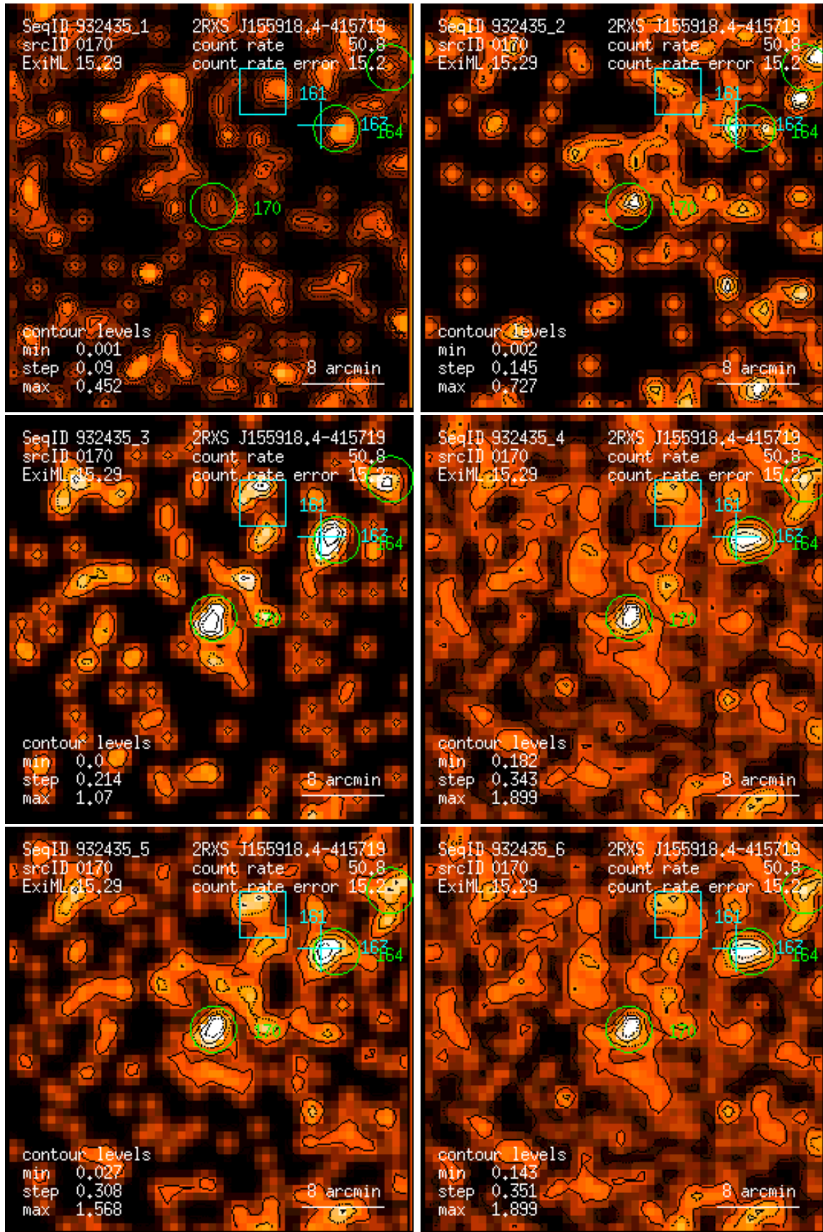
Figure 170: RASS 932435: detection 0170: band rate images, Gaussian filter: (1) PSPC channels 11 – 41, (2) 52 – 90, (3) 91 – 201, (4) 11 – 235, (5) 52 – 201, (6) 11 – 201. Broad band rates in counts/ks. Band rate contour levels in counts/ks/arcmin 2 .
