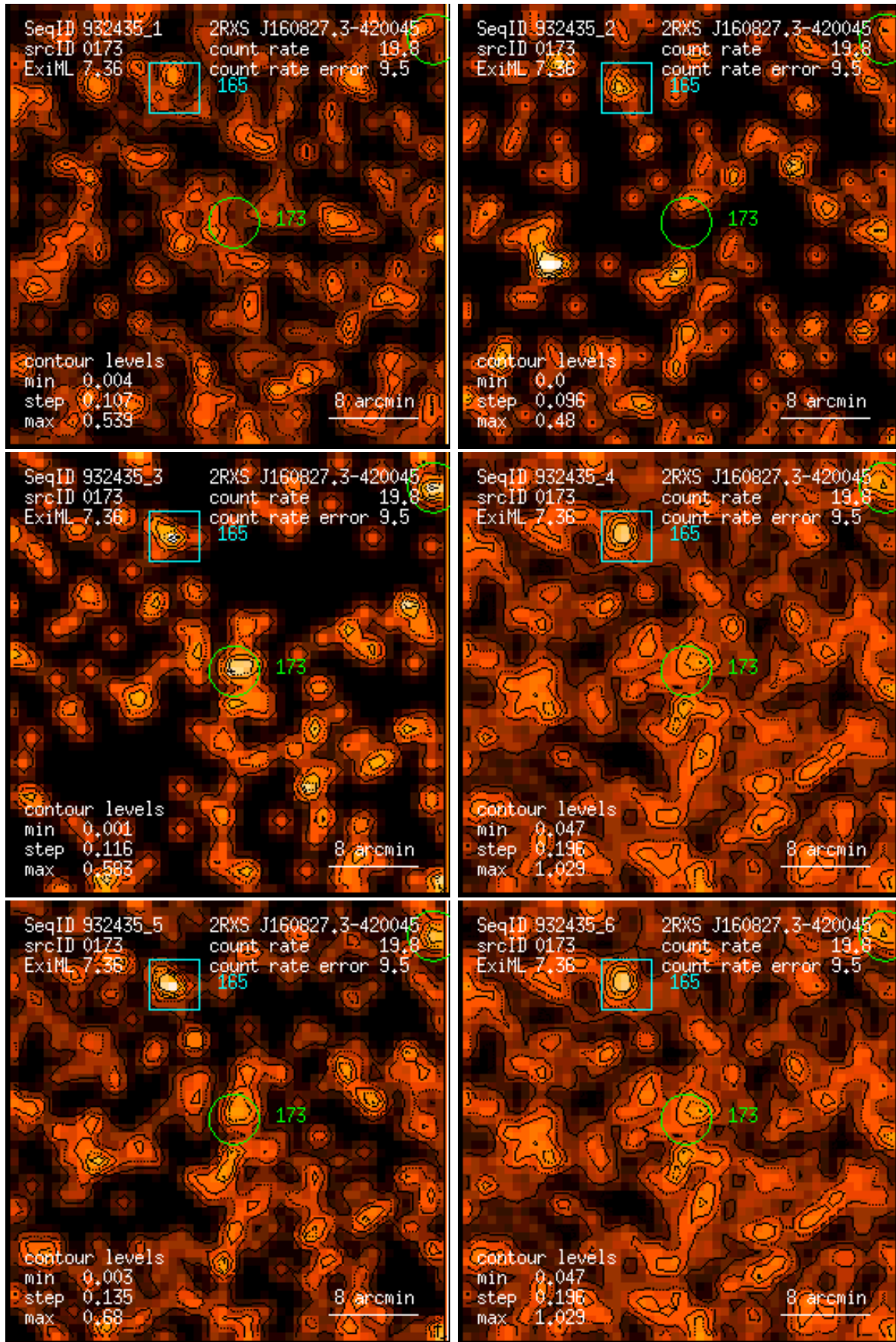
Figure 173: RASS 932435: detection 0173: band rate images, Gaussian filter: (1) PSPC channels 11 – 41, (2) 52 – 90, (3) 91 – 201, (4) 11 – 235, (5) 52 – 201, (6) 11 – 201. Broad band rates in counts/ks. Band rate contour levels in counts/ks/arcmin 2 .
