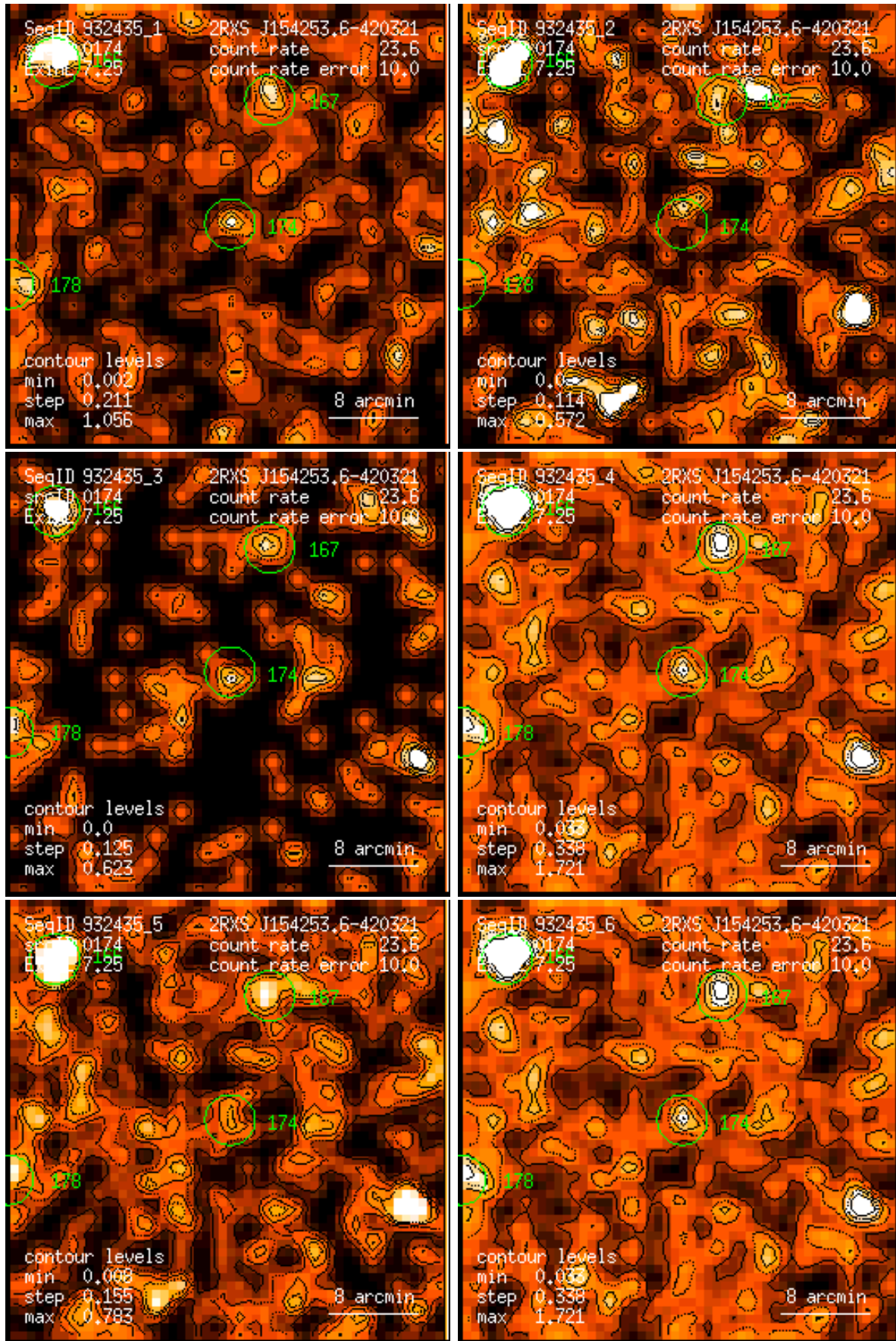
Figure 174: RASS 932435: detection 0174: band rate images, Gaussian filter: (1) PSPC channels 11 – 41, (2) 52 – 90, (3) 91 – 201, (4) 11 – 235, (5) 52 – 201, (6) 11 – 201. Broad band rates in counts/ks. Band rate contour levels in counts/ks/arcmin 2 .
