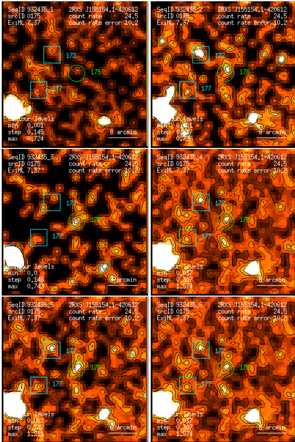
Figure 175: RASS 932435: detection 0175: band rate images, Gaussian filter: (1) PSPC channels 11 – 41, (2) 52 – 90, (3) 91 – 201, (4) 11 – 235, (5) 52 – 201, (6) 11 – 201. Broad band rates in counts/ks. Band rate contour levels in counts/ks/arcmin 2 .
