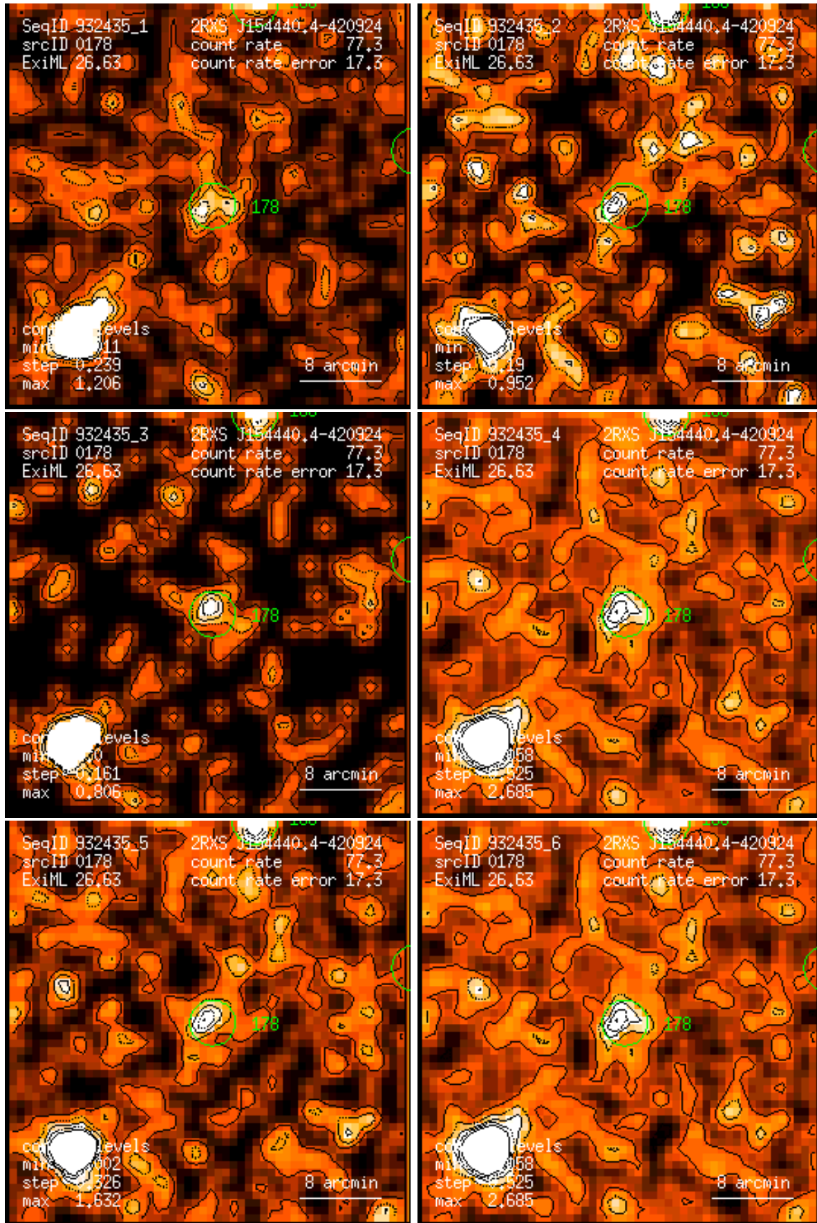
Figure 178: RASS 932435: detection 0178: band rate images, Gaussian filter: (1) PSPC channels 11 – 41, (2) 52 – 90, (3) 91 – 201, (4) 11 – 235, (5) 52 – 201, (6) 11 – 201. Broad band rates in counts/ks. Band rate contour levels in counts/ks/arcmin 2 .
