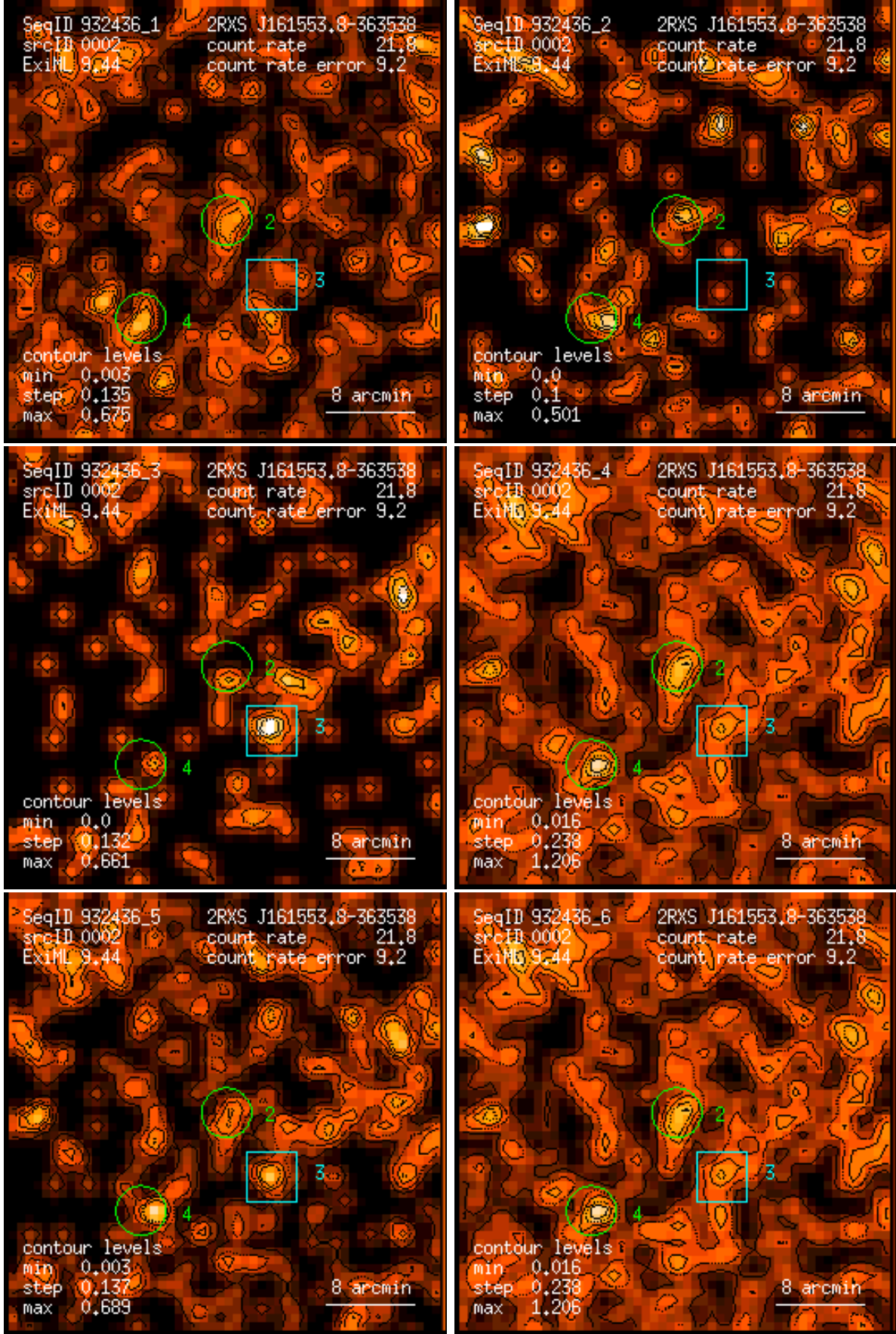
Figure 2: RASS 932436: detection 0002: band rate images, Gaussian filter: (1) PSPC channels 11 – 41, (2) 52 – 90, (3) 91 – 201, (4) 11 – 235, (5) 52 – 201, (6) 11 – 201. Broad band rates in counts/ks. Band rate contour levels in counts/ks/arcmin 2 .
