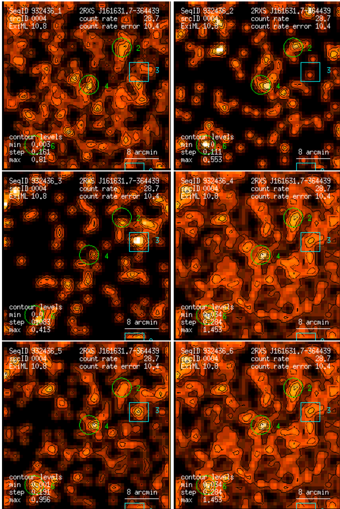
Figure 4: RASS 932436: detection 0004: band rate images, Gaussian filter: (1) PSPC channels 11 – 41, (2) 52 – 90, (3) 91 – 201, (4) 11 – 235, (5) 52 – 201, (6) 11 – 201. Broad band rates in counts/ks. Band rate contour levels in counts/ks/arcmin 2 .
