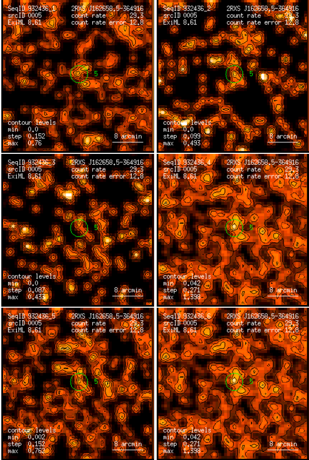
Figure 5: RASS 932436: detection 0005: band rate images, Gaussian filter: (1) PSPC channels 11 – 41, (2) 52 – 90, (3) 91 – 201, (4) 11 – 235, (5) 52 – 201, (6) 11 – 201. Broad band rates in counts/ks. Band rate contour levels in counts/ks/arcmin 2 .
